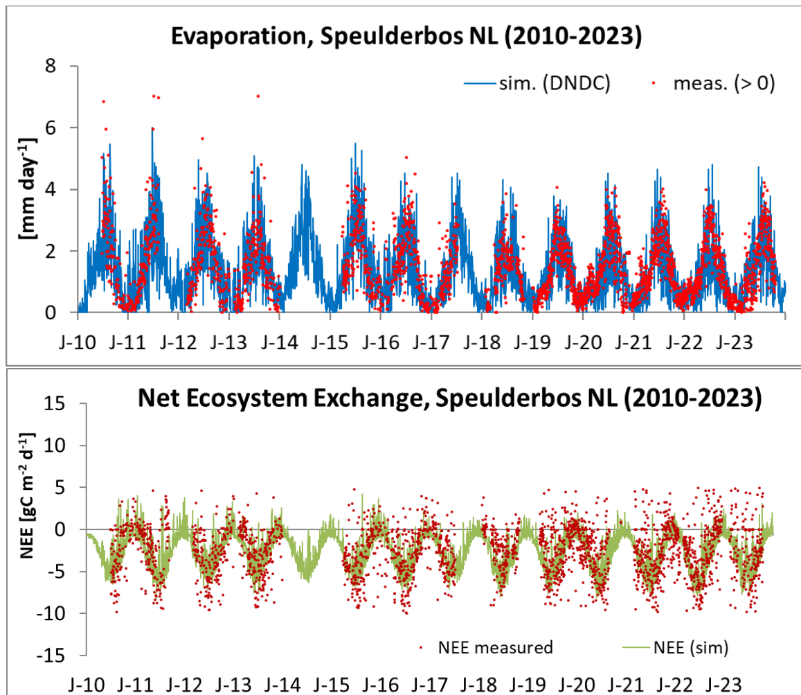
Figure T: Preliminary comparison of measured and simulated daily Evaporation (top) and NEE (bottom) throughout 11 consecutive years.
