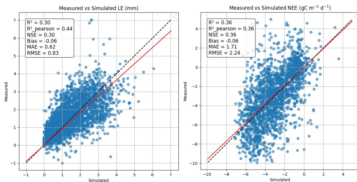
Figure U: Preliminary statistical relations between simulated and measured fluxes
