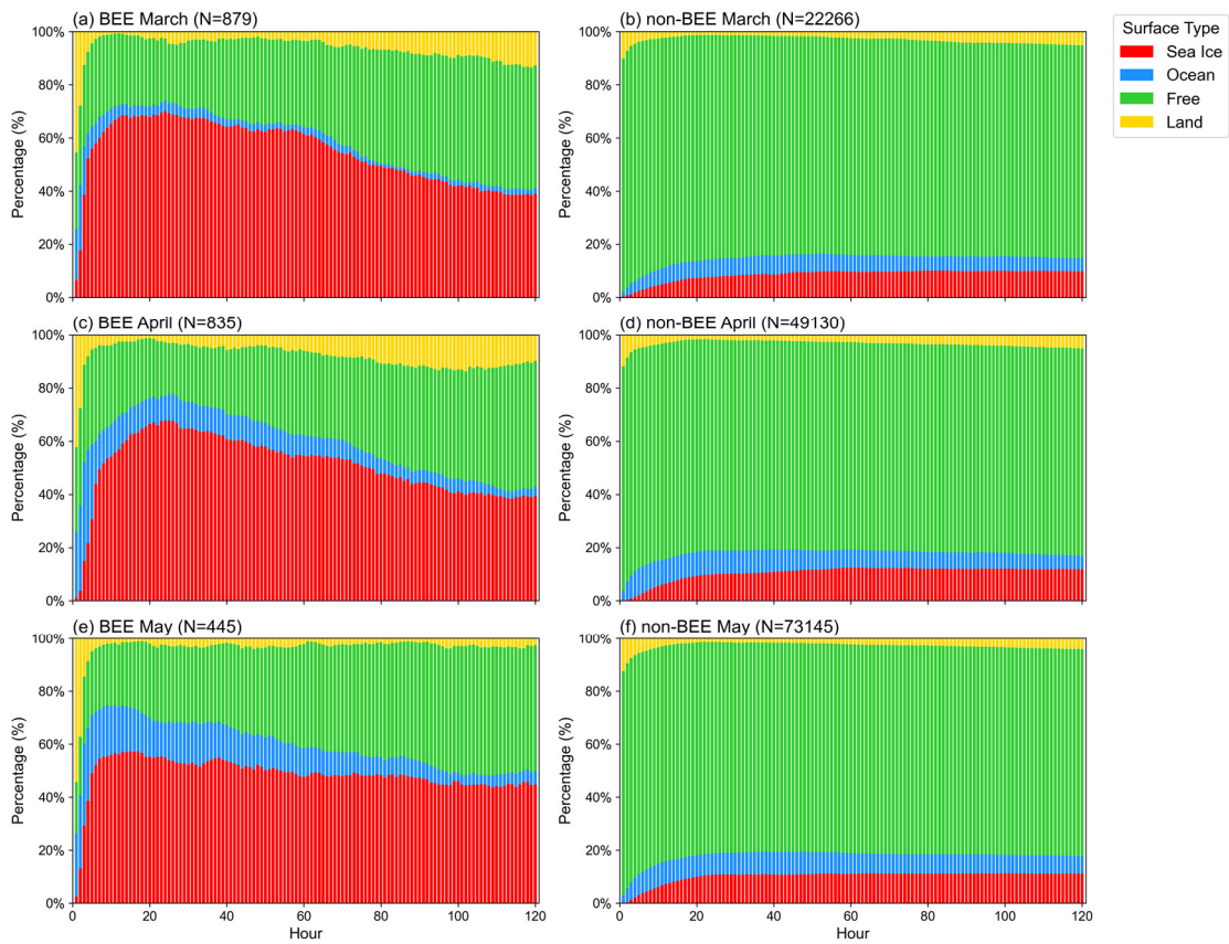
600 Figure 11. Percentage of air mass contact times with sea ice, open ocean, free troposphere and land along the 5-d backward trajectories during the identified BEEs and non-BEEs in Ny-Ålesund in March (a, b), April (c, d), and May (e, f) for the period of 2017 to 2023. The number N in each panel represents the monthly cumulative total of hours for air mass in each 200 m altitude interval within the 0–3 km range.
