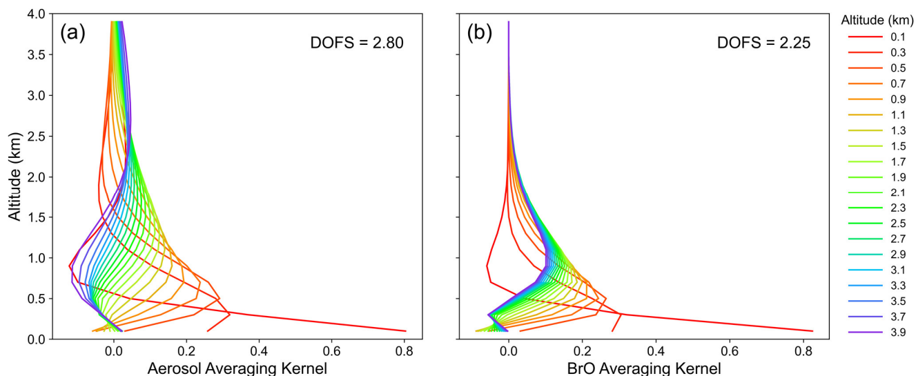
225 Figure 2. Averaging kernels for aerosol (a) and BrO (b) at 10:22 UTC on April 2, 2020. The AOD is 7.73 \times 10^{-2} . The DOFS are 2.80 for the aerosol extinction profile and 2.25 for the BrO profile. Curves of different colours represent the averaging kernels at different altitude layers.
