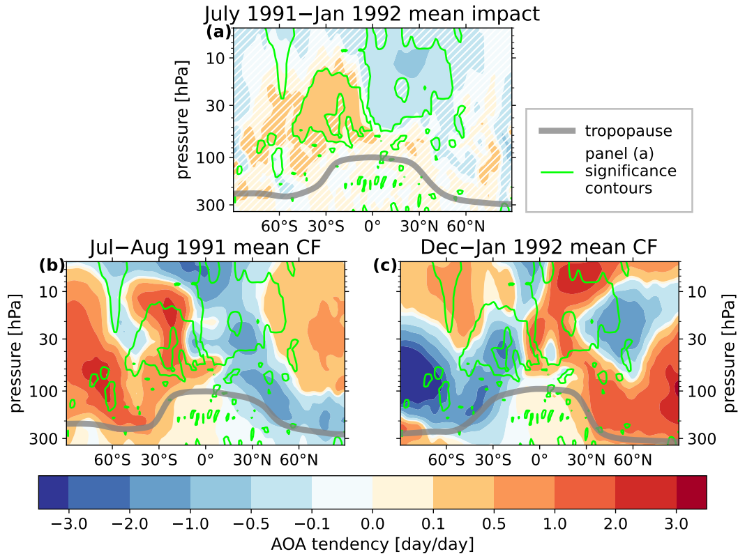
Figure 11. Demonstration-Indication of the hypothesized BDC seasonal cycle damping during the first 8 months of the volcanic experiments, in terms of the AoA tendency in day/day. (a) the ensemble-mean impact, averaged between July 1 1991 and Jan 1 1992. A green contour is drawn at 95% significance, and regions of insignificance are filled with white hatching. (b) the summertime CF ensemble-mean, averaged between July 1 1991 and August 1 1991. (c) the wintertime CF ensemble mean, averaged between Dec 1 1991 and Jan 1 1992. In all panels, a thick grey line shows the tropopause averaged over the same period. In panels (b) and (c), the thin green significance contour from panel (a) is reproduced for visual reference.
