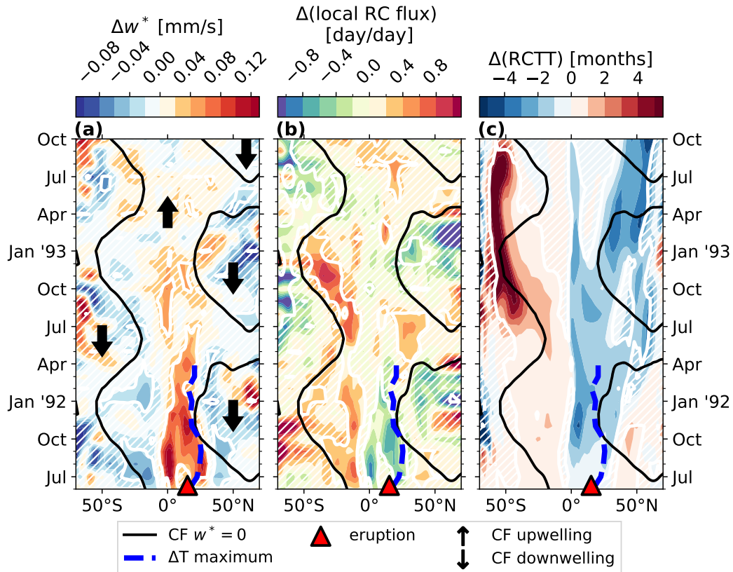
Figure 10. Relationship between the ensemble-mean impacts in vertical residual velocity, and aging by transport-residual circulation advection at 30 hPa from July 1991 to January-October 1993. In all panels, solid black contours are drawn at w^* = 0 in the CF ensemble mean, a thick dashed blue line shows the latitude of maximum \Delta T from July 1991 to April 1992, and a red triangle shows the position of the Mt. Pinatubo eruption. White contours are drawn at 95% significance, and regions of insignificance are filled with white hatching. (a) \Delta w^* in \text{mm s}^{-1} . Thick black arrows show regions of upwelling and downwelling in the CF data. (b) impact in AoA local transport-residual circulation advective flux (Eq. (5) + Eq. (6)) in days per day. (c) RCTT impact in months.
