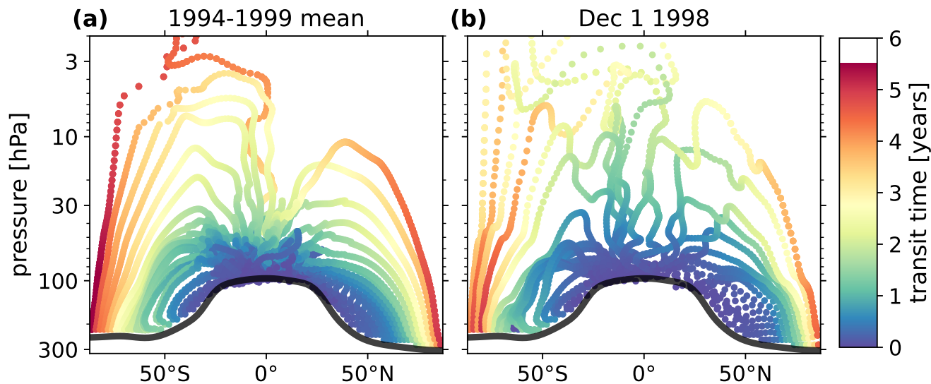
Figure 4. Select single-member (CF ensemble-mean ensemble member 9 ) RCTT trajectories for gridpoints near the tropopause, every 2^\circ in latitude, from 20^\circ – 90^\circ on each side of the equator. (a) the 5-year mean trajectories (b) the trajectories computed on Dec 1 1998. The colors indicate the transit time along the trajectories. Note that visually discontinuous trajectories near the tropical tropopause are visible in panel (a). These features are an artifact of the trajectory averaging, due to the fact that the individual trajectories become highly variable in that region. These artifacts are not present in the individual member trajectories, and are purely visual, meaning that they do not affect the ensemble-mean RCTT in any way.
