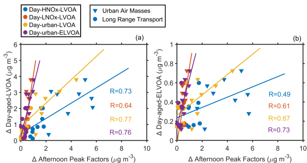
1060 Figure 7. Correlation between the enhancement of (a) Day-aged-LVOA and afternoon peak factors 1061 and (b) Day-aged-ELVOA and afternoon peak factors. Afternoon peak factors include Day-HNO x - 1062 LVOA, Day-LNO x -LVOA, Day-urban-LVOA, and Day-urban-ELVOA. For afternoon peak factors, 1063 the enhancement ( \Delta ) was regarded as the average mass concentration during 00:00-6:00 LT and 1064 12:00-18:00 LT. For Day-aged-LVOA and Day-aged-ELVOA, the enhancement ( \Delta ) was estimated 1065 as the difference between average mass concentration during 00:00-6:00 LT and 12:00-18:00 LT.
