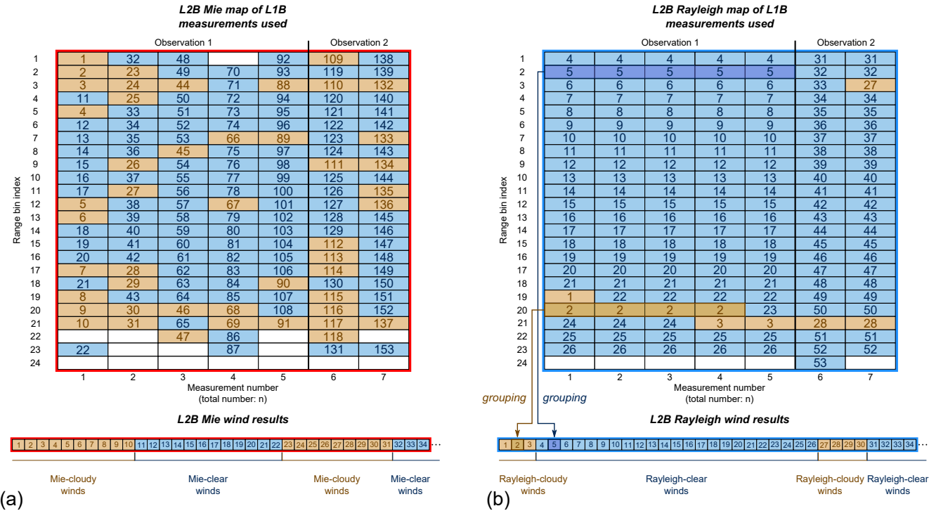
Figure A2. Schematic illustrating the grouping algorithm for (a) Mie winds and (b) Rayleigh winds in the Aeolus L2B processor. Individual L1B measurements, per range bin and observation, are classified as "cloudy" or "clear" and then gathered into groups according to the mission parameter settings. These groups are alternately stacked into a one-dimensional array in the L2B product, with L2B wind results enumerated following the order of measurements within each observation. The example shown is based on L1B and L2B data from orbit 21857 (1 June 2022, 05:49–07:19 UTC) with P/N settings 114/5. For other P/N settings, multiple L1B measurements may contribute to a single L2B Mie wind result. Due to the longer accumulation length of Rayleigh winds, multiple L1B measurements contribute to a single Rayleigh wind result even for P/N 114/5, as exemplified for wind result 2 (Rayleigh-cloudy) and wind result 5 (Rayleigh-clear).
