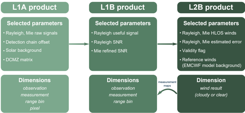
Figure A1. Overview of the L1A, L1B, and L2B product parameters analysed in this study, together with their respective dimensions. The dimensions indicate the number of elements at each processing level, e.g. measurements and observations (horizontal scale), range bins (vertical scale), and retrieved wind results (including horizontal and vertical scales).
