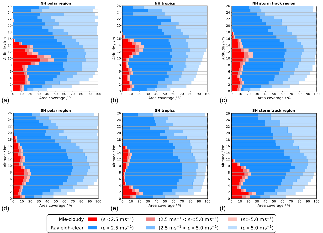
Figure C1. Aeolus Mie-cloudy (reds) and Rayleigh-clear (blues) global wind data coverage on 20 July 2019 in different geographical regions: (a) NH polar region (latitude > 60^\circ\text{N} ); (b) NH tropics ( 0^\circ < \text{latitude} < 20^\circ\text{N} ); (c) NH storm track region ( 40^\circ\text{N} < \text{latitude} < 60^\circ\text{N} ); (d) SH polar region (latitude > 60^\circ\text{S} ); (e) SH tropics ( 0^\circ < \text{latitude} < 20^\circ\text{S} ); (f) SH storm track region ( 40^\circ\text{S} < \text{latitude} < 60^\circ\text{S} ). The colour shading indicates the proportion of data within specific intervals of the absolute value of (O-B) wind speed difference \varepsilon . The Rayleigh-clear wind error is normalised to a vertical bin thickness of 1 km.
