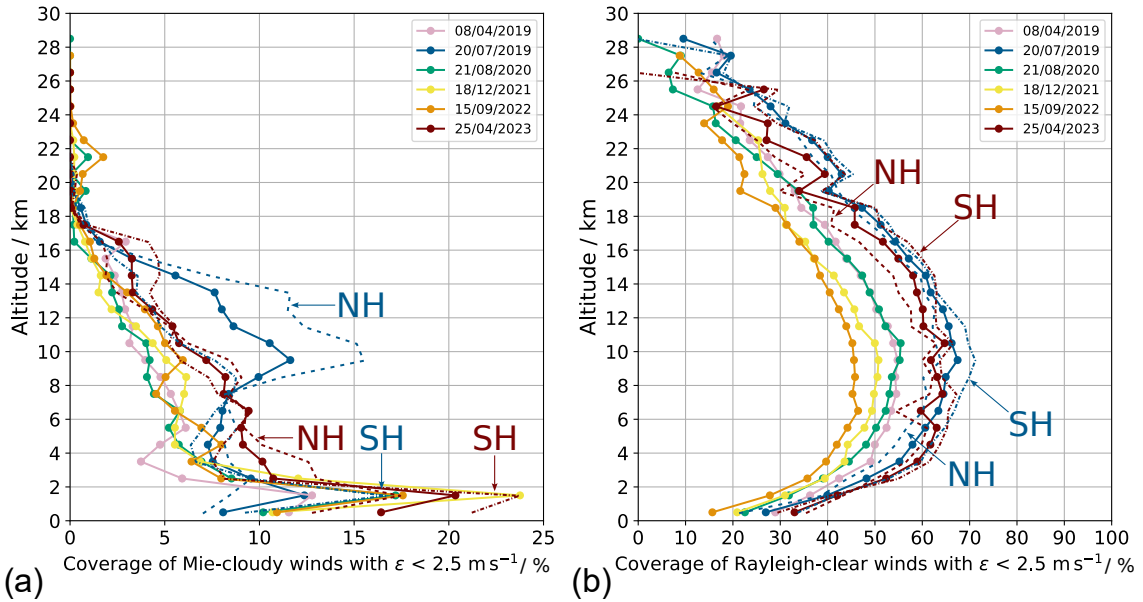
Figure 6. Altitude dependence of (a) L2B Mie-cloudy and (b) L2B Rayleigh-clear wind data coverage with (O-B) wind speed difference \epsilon < 2.5 \text{ m s}^{-1} for six selected days throughout the mission period. The Rayleigh-clear wind error is normalised to a vertical bin thickness of 1 km. For 20 July 2019 and 25 April 2023, the data are additionally shown separately for the NH (dashed lines) and SH (dash-dotted lines).
