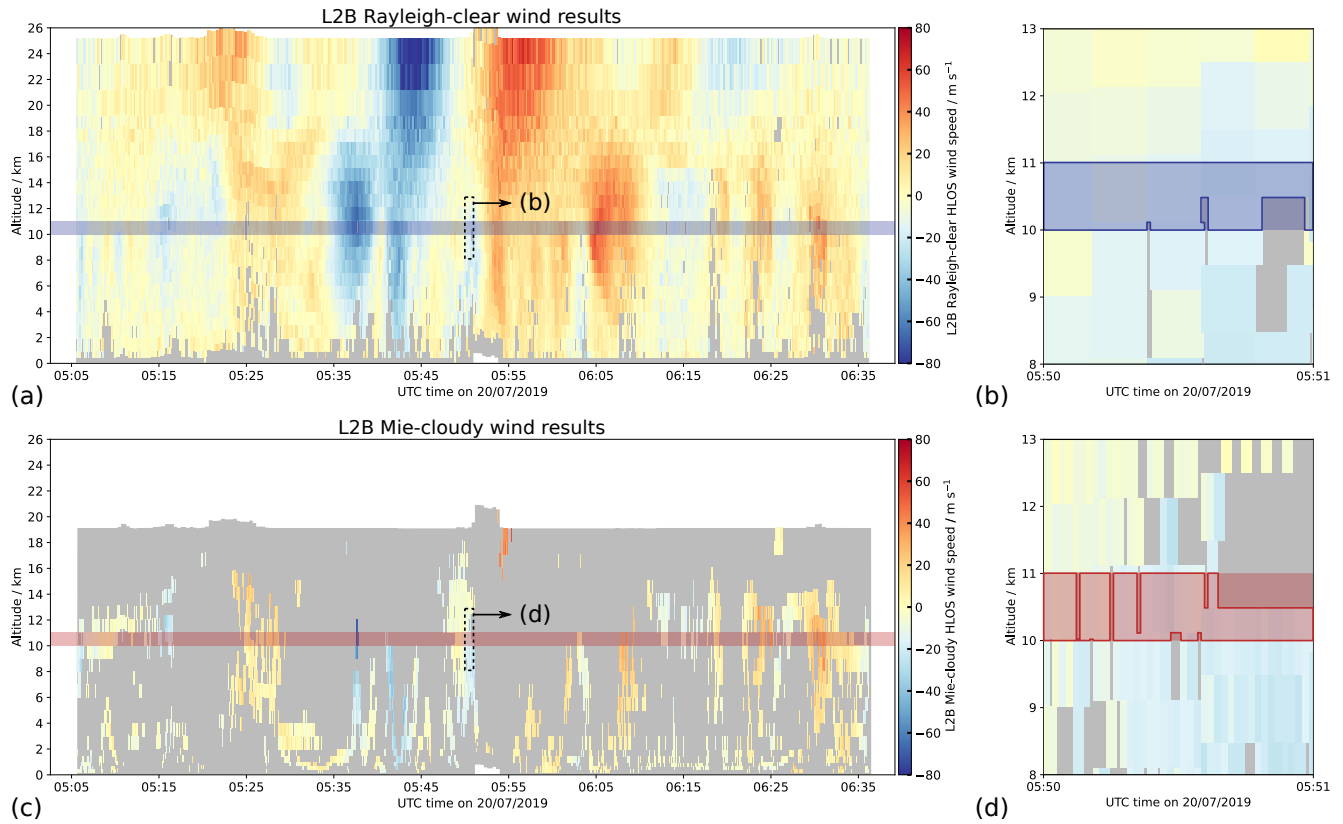
Figure 4. (a, b) Aeolus L2B Rayleigh-clear and (c, d) Mie-cloudy HLOS wind results measured on 20 July 2019 between 05:05 UTC and 06:36 UTC (orbit number 5254). The grey-shaded area indicates invalid data. Together with the coloured valid wind data, it shows the overall coverage of the L2B data grid for both channels. Coverage is determined per 1 km altitude range by calculating the ratio of the area containing wind results—outlined in blue and red in panels (b) and (d)—to the total area spanned over that altitude range.
