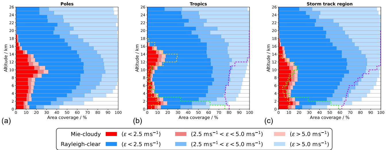
Figure 7. Aeolus Mie-cloudy (reds) and Rayleigh-clear (blues) global wind data coverage on 20 July 2019 in different geographical regions: (a) poles (latitude > 60^{\circ}\text{N/S} ); (b) tropics (latitude < 20^{\circ}\text{N/S} ); (c) storm track region ( 40^{\circ}\text{N/S} < \text{latitude} < 60^{\circ}\text{N/S} ). The colour shading indicates the proportion of data within specific intervals of the absolute value of (O-B) wind speed difference \epsilon . The Rayleigh-clear wind error is normalised to a vertical bin thickness of 1 km. The dashed lines in panels (b) and (c) represent pre-launch LIPAS simulations of the coverage from clouds (orange), aerosols (green) and molecules (purple), adapted from Marseille et al. (2001) . Corresponding data for the polar regions are not available.
