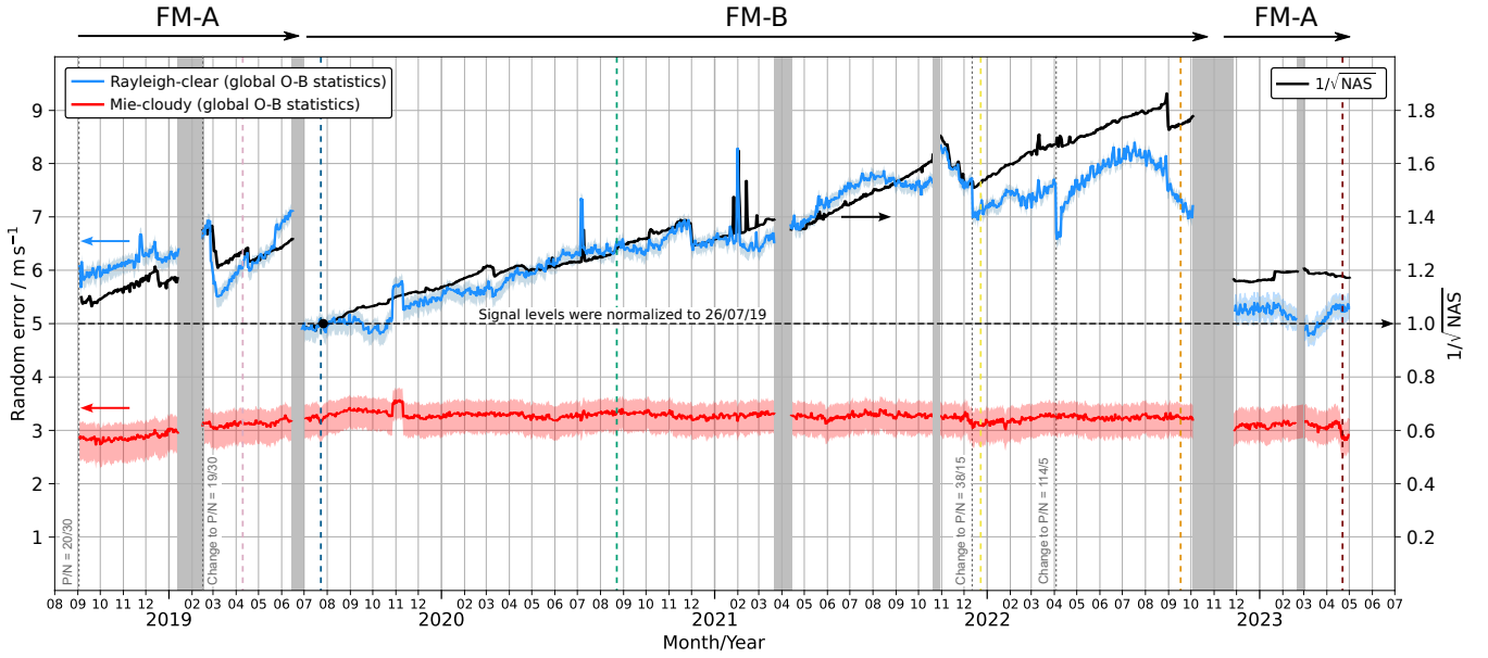
Figure 2. Timeline of the global, daily average random error for Aeolus Rayleigh-clear (blue) and Mie-cloudy (red) wind observations over the mission period, derived from (O–B) statistics assuming a model background error of 2.0 \text{ m s}^{-1} . Shaded areas indicate the uncertainty range corresponding to assumed model background errors of 1.5 \text{ m s}^{-1} (upper bound) and 2.5 \text{ m s}^{-1} (lower bound). The black line (right axis) shows the reciprocal square root of the atmospheric signal level ( 1/\sqrt{\text{NAS}} ), normalised to its value on 26 July 2019. Grey-shaded regions indicate periods when the instrument was temporarily switched off. Coloured vertical dashed lines mark specific days selected for analysis in this study.
