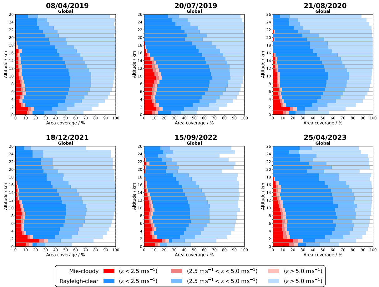
Figure 5. Aeolus Mie-cloudy (reds) and Rayleigh-clear (blues) global wind data coverage for selected days throughout the mission period. Mie-cloudy coverage is overlaid on top of the Rayleigh-clear coverage. The colour shading indicates the proportion of data within specific intervals of the (O-B) wind speed difference \epsilon relative to the ECMWF model background, assuming a background error of 2.5 \text{ m s}^{-1} . The Rayleigh-clear wind error is normalised to a vertical bin thickness of 1 km.
