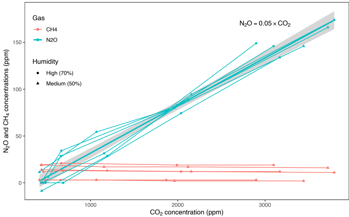
Figure 5: Testing the cross-sensitivity of CH 4 and N 2 O concentrations with increasing CO 2 levels. While CH 4 was insensitive to CO 2 , N 2 O readings increased by 0.05 ( \pm 0.002 SE) ppm per ppm of CO 2 , regardless of humidity levels.
