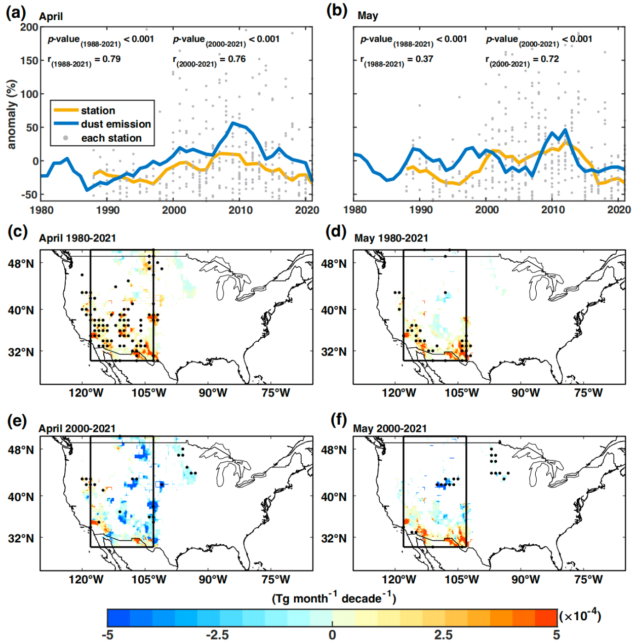
318 Figure 3. Changes in North American dustiness in April and May during 1980-2021 and
