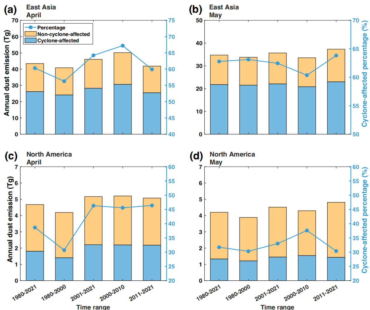
Figure 10. Regime shifts in extratropical cyclone-affected dust emissions (Tg) across East Asia and North America during April and May for multiple subperiods within 1980-2021. The annual average dust emissions (Tg) along the passage of extratropical cyclones (blue bars) and those unaffected by them (yellow bars) are shown for (a, b) East Asia and (c, d) North America in (a, c) April and (b, d) May, for the time periods: 1980-2021, 1980-2000, 2001-2021, 2000-2010, and 2011-2021, with reference to the left y-axis. The blue bars show the cyclone-affected dust emissions, defined as the difference between total dust emissions and the emissions in the cyclone-controlled experiments (i.e., total - cyclone-controlled), while the yellow bars show the emissions estimated from the cyclone-controlled experiments. The blue solid line represents the percentage of dust emissions affected by extratropical cyclones (%) over these periods, corresponding to the right y-axis.
