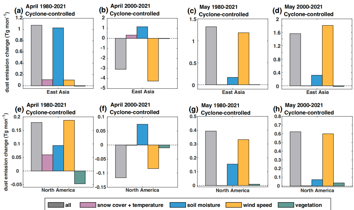
Figure 11. Changes in East Asian and North American dust emission ( \text{Tg month}^{-1} ) and the contribution of several environmental variables during 1980-2021 in cyclone-controlled experiments. Figure elements are identical to those in Fig. 4.
