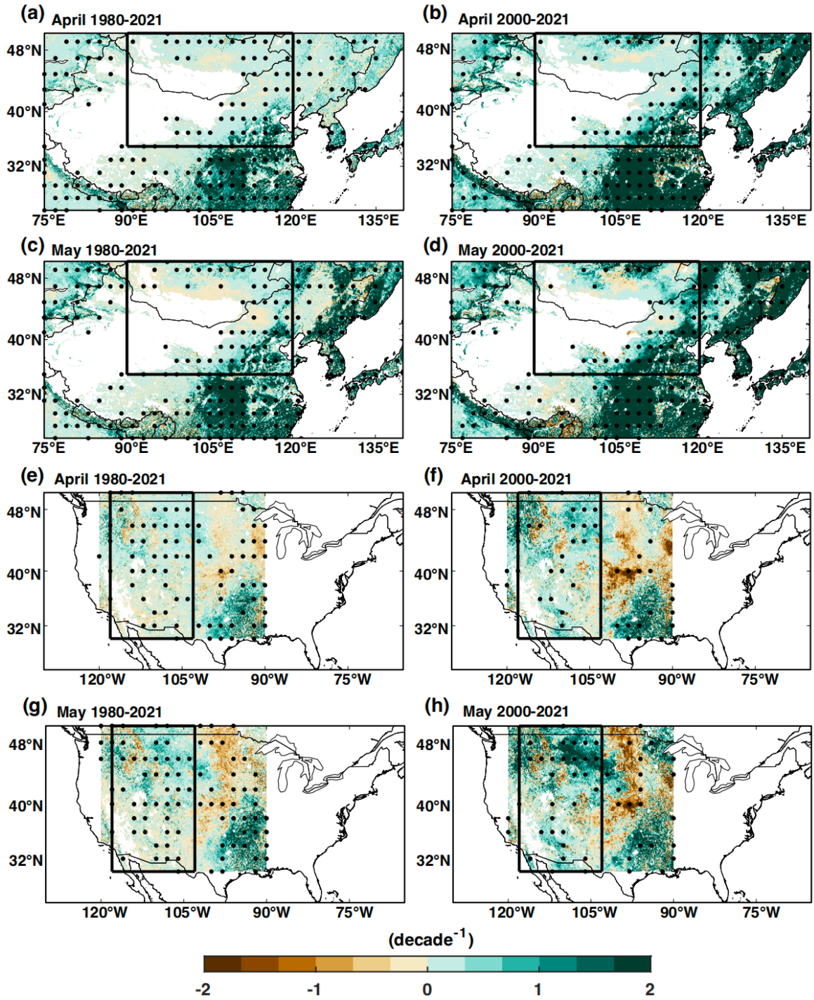
Figure 7. Changes in LAI in April and May for the period 1980-2021 and 2000-2021. Trends in (a, b) April and (c, d) May LAI (decade -1 ) across East Asia for the period (a, c) 1980-2021 and (b, d) 2000-2021. Trends in (e, f) April and (g, h) May daily LAI (decade -1 ) across North America for the period (e, g) 1980-2021 and (f, h) 2000-2021, respectively. Black dots indicate significant ( p -values < 0.1, based on the Mann-Kendall trend test) trend.
