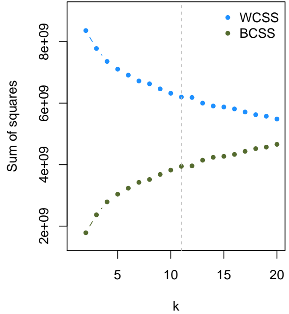
Figure 2. In the k -means algorithm, the user has to provide k . We employed commonly used elbow criteria for two metrics as a function of k a) change in WCSS and b) change in BCSS. The optimal k is the smallest number of compact and separable clusters.
