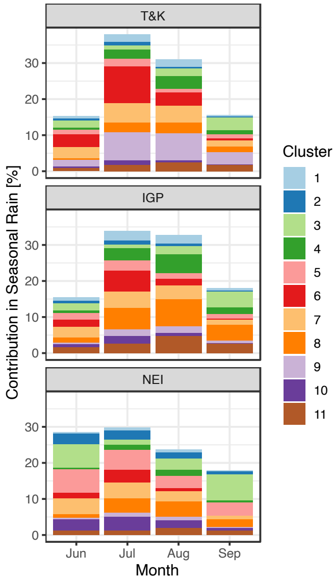
Figure 8. The monthly contributions of each cluster (stacked color strips) and total (total height of the bars) are shown as percentages of seasonal rainfall in K&T&K, IGP, and NEI regions.
