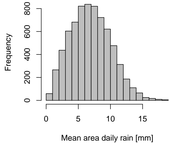
Figure 1. The frequency distribution of daily area mean rainfall for the study region is normally distributed with approximately 1% of days with no rain in the domain during JJAS. Therefore, all the days were clustered.
