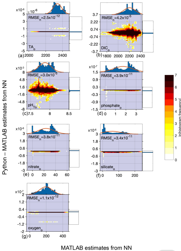
Figure 6. Difference between Python and MATLAB neural network estimates (y axis) compared to MATLAB estimates (x axis) for open ocean (o) data and all equations combined for TA (a, 4 899 512 total estimates from all equations), DIC (b, 5 497 004 estimates), \text{pH}_T (c, 3 188 864 estimates), phosphate (d, 12 228 432 estimates), nitrate (e, 12 228 432 estimates), silicate (f, 12 228 432 estimates), and oxygen (g, 12 228 560 estimates); n = 306\,227 for TA, 343 580 for DIC, 199 304 for \text{pH}_T , and 764 301 for phosphate, nitrate, silicate, and oxygen. All units, except for \text{pH}_T , are \mu\text{mol kg}^{-1} . Top and side histograms represent the distribution of the x and y axes, respectively. Note the differences in the x- and y-axis scales. \text{RMSE}_n is the normalized root mean square error, or the RMSE divided by the mean of all estimates from MATLAB_NN.
