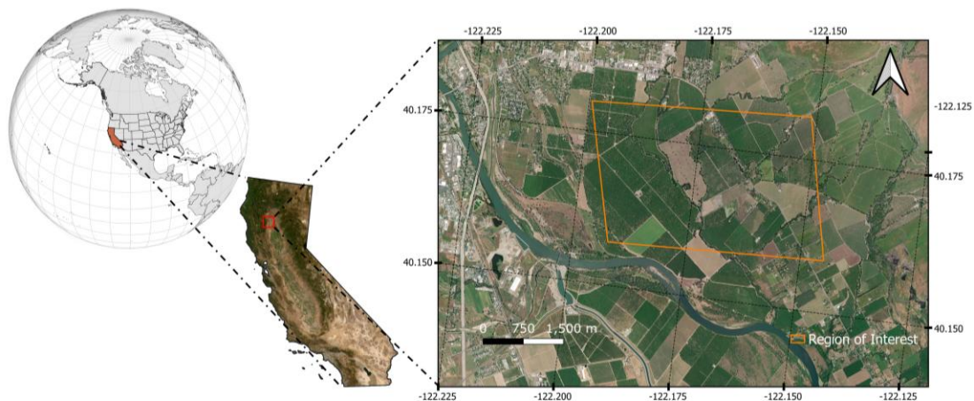
Actual Evapotranspiration: OpenET Vs sDRIPS for California
