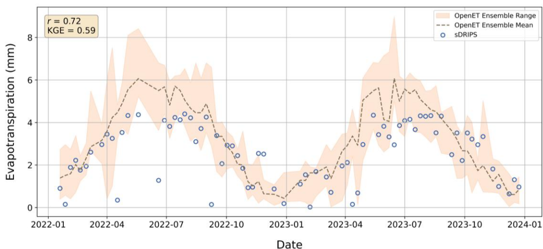
545 Fig. 9: Location of the region of interest in California with the timeseries of estimates from OpenET and sDRIPS-based SEBAL ET. Satellite basemap from ESRI.
