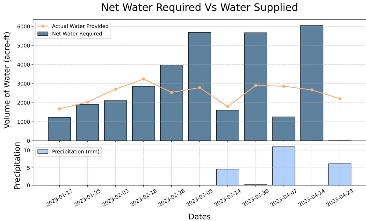
Fig. 8: Timeseries of net water required by TBP vs amount of water supplied to TBP. TBP operates from January to April each year; outside this period, fields rely mainly on rainfall.
