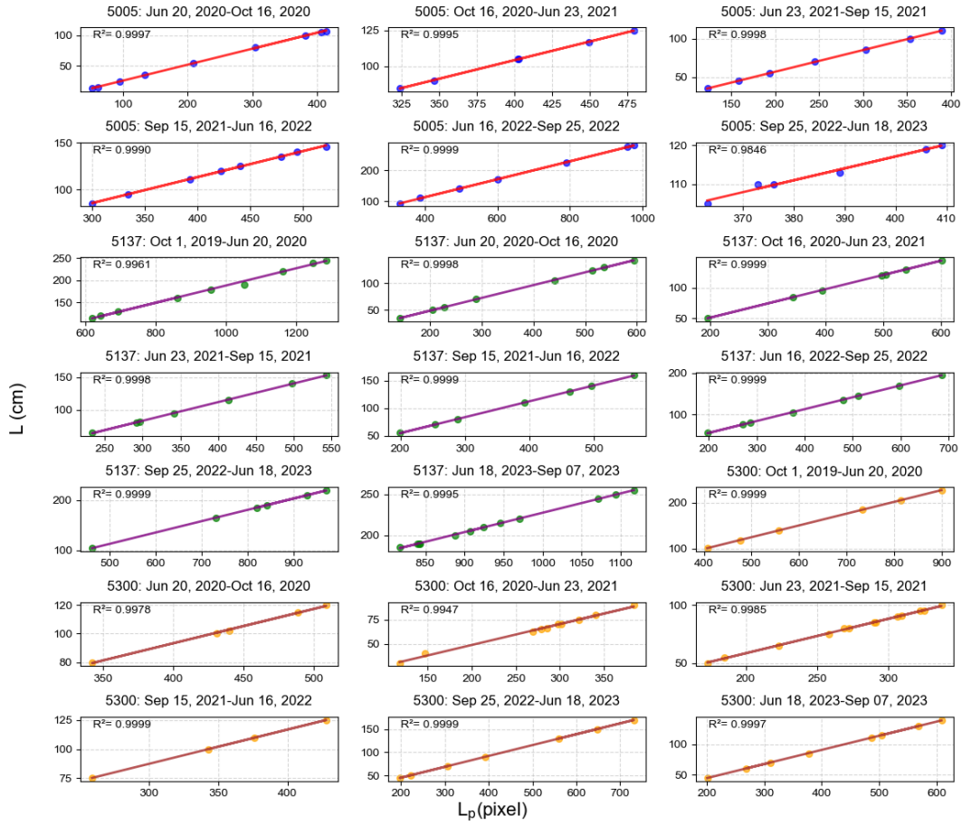
Figure S1 Linear relationship between L_p and L for each monitoring period at each monitoring site.
