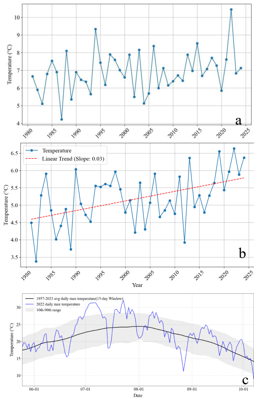
Figure S3 Variation of mean EAR-land air temperature in July(a) and July-September (b) at the corresponding grid of Kangxiwa Glacier during the period from 1981 to 2024. (c) Comparison of June-September daily max air temperature in 2022 with the 1957-2023 mean at Taxkorgan.
