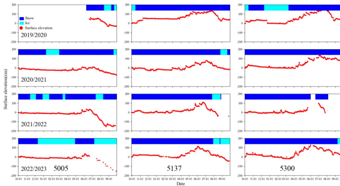
Figure S2 The surface elevation changes at three locations on the Kangxiwa Glacier and their evolutions of snow and bare ice surface conditions.
