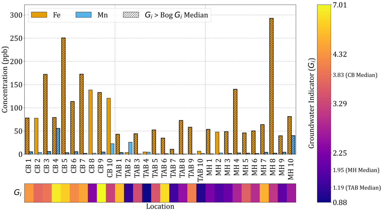
510 Figure 9: Concentrations of iron (Fe, orange) and manganese (Mn, blue) trace elements and a heatmap of associated groundwater indicator ( G_i ) variables for the thirty surface water samples collected from Caribou Bog (CB), Thousand Acre Bog (TAB), and Meddybemps Heath (MH). Samples collected at zones with G_i values greater than the bog G_i median value are denoted with hatch marks to compare with associated trace element concentrations.
