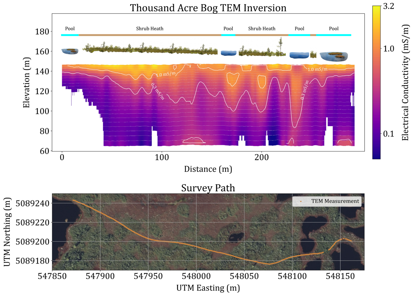
355 Figure 4: Transient electromagnetic induction (TEM) electrical conductivity (mS/m) inversion results from surveys conducted in Thousand Acre Bog, indicating variations in the electrical conductivity structures beneath the patterned pools and correspondence to surficial vegetation patterning (Davis & Anderson, 1999). Sensitivity of the TEM inversion was filtered using a standard deviation of less than four to remove low sensitivity portions of the model (white). Basemap data from © Microsoft (2024).
