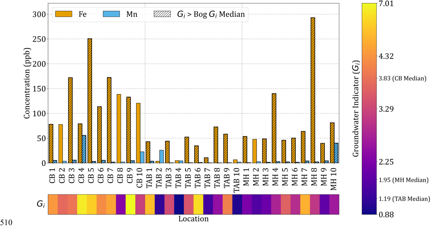
Figure 9: Concentrations of iron (Fe, orange) and manganese (Mn, blue) trace elements and a heatmap of associated groundwater indicator ( G_i ) variables for the thirty surface water samples collected from Caribou Bog (CB), Thousand Acre Bog (TAB), and Meddybemps Heath (MH). Samples collected at zones with G_i values greater than the bog G_i median value are denoted with hatch marks to compare with associated trace element concentrations.
