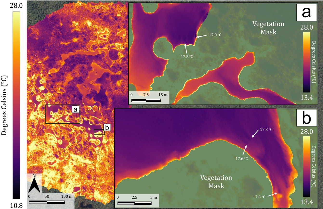
Figure 7: Uncrewed aerial system (UAS) Thermal Infrared (TIR) orthomosaic map of Caribou Bog patterned pools captured on June 9 th , 2023, and calibrated against the thermal emissivity of water. Discrete points of cooler water are highlighted in the (a) the
