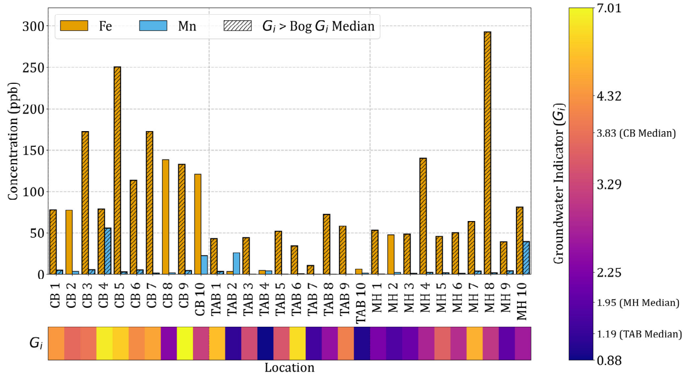
Figure 9: Concentrations of iron (Fe, orange) and manganese (Mn, blue) trace elements and a heatmap of associated groundwater indicator ( G_i ) variables for the thirty surface water samples collected from Caribou Bog (CB), Thousand Acre Bog (TAB), and Meddybemps Heath (MH). Samples collected at zones with G_i values greater than the bog G_i median value are denoted with hatch marks to compare with associated trace element concentrations.
