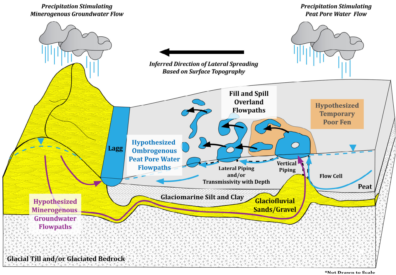
Figure 10: Conceptual hydrogeologic model of ombrogenous and minerogenous flows to patterned pools, Precipitation is shown to stimulate both ombrogenous and minerogenous groundwater flowpaths. Shallow minerogenous groundwater flowpaths would discharge to the lagg in the system. The deepest minerogenous groundwater flowpaths occur through the glaciofluvial aquifer and result in vertical flows to pools immediately above or adjacent to the aquifer connection. Minerogenous groundwater contributions to pools would result in a temporary change in peatland type. Ecology on the surface may potentially show characteristics of a poor fen around pools local to the esker. Ombrogenous flow cells of peat pore water (Reeve et al., 2009) are shown to originate from the center of the bog, driven by the topography and permeability of the underlying mineral sediments, causing vertical flow to the pool immediately above or adjacent to the esker. Both forms of vertical flux to the pools would result in enhanced lateral transmissivity via piping or peat matrix flow in the subsurface. Additionally, when the pools up topographic gradient reach storage capacity, fill and spill overland flow may also be observed between pools. These chain reactions in changes of flow would subsequently enhance lateral spreading of the pool system.
