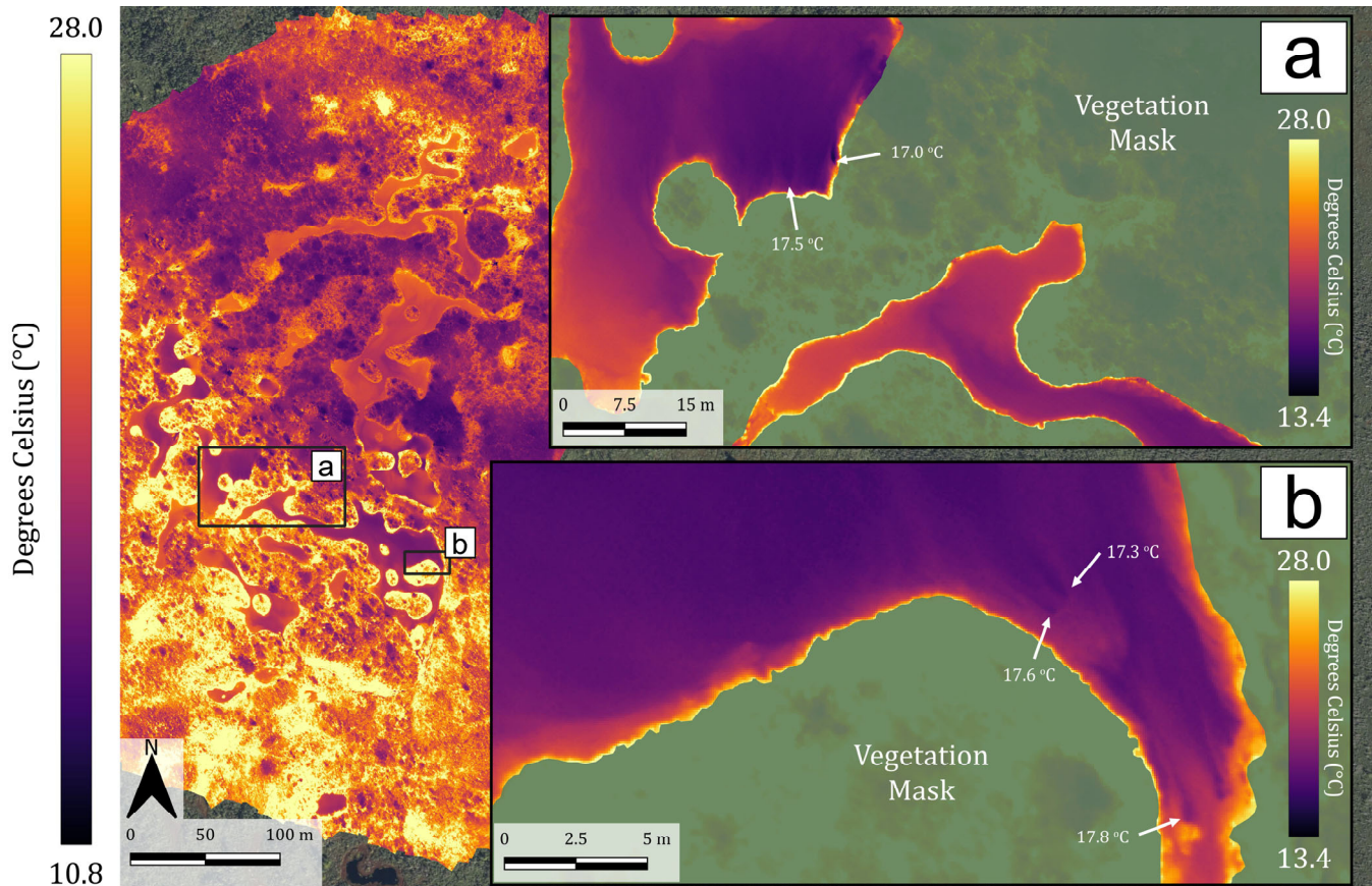
Figure 7: Uncrewed aerial system (UAS) Thermal Infrared (TIR) orthomosaic map of Caribou Bog patterned pools captured on June 9 th , 2023, and calibrated against the thermal emissivity of water (left, 10.8 °C to 28.0 °C). Discrete points of cooler water are
