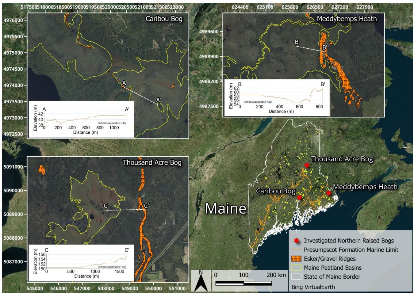
Figure 1: Images (© Microsoft) of Caribou Bog (central unit), Thousand Acre (Crystal) Bog, and Meddybemps Heath (southern unit) in Maine (USA) with mapped nearby mapped glaciofluvial eskers/gravel deposits (Newman, 1980; Cameron et al., 1984; Shreve, 1985; Thompson & Borns, 1985). Elevation profiles (white) from the State of Maine (2020) between the patterned pools investigated and the nearest esker/gravel deposits are presented for the three peat bogs. All images are displayed using the WGS 84 / UTM Zone 19N (EPSG 32619) coordinate reference system, and tick marks are distances in meters.
