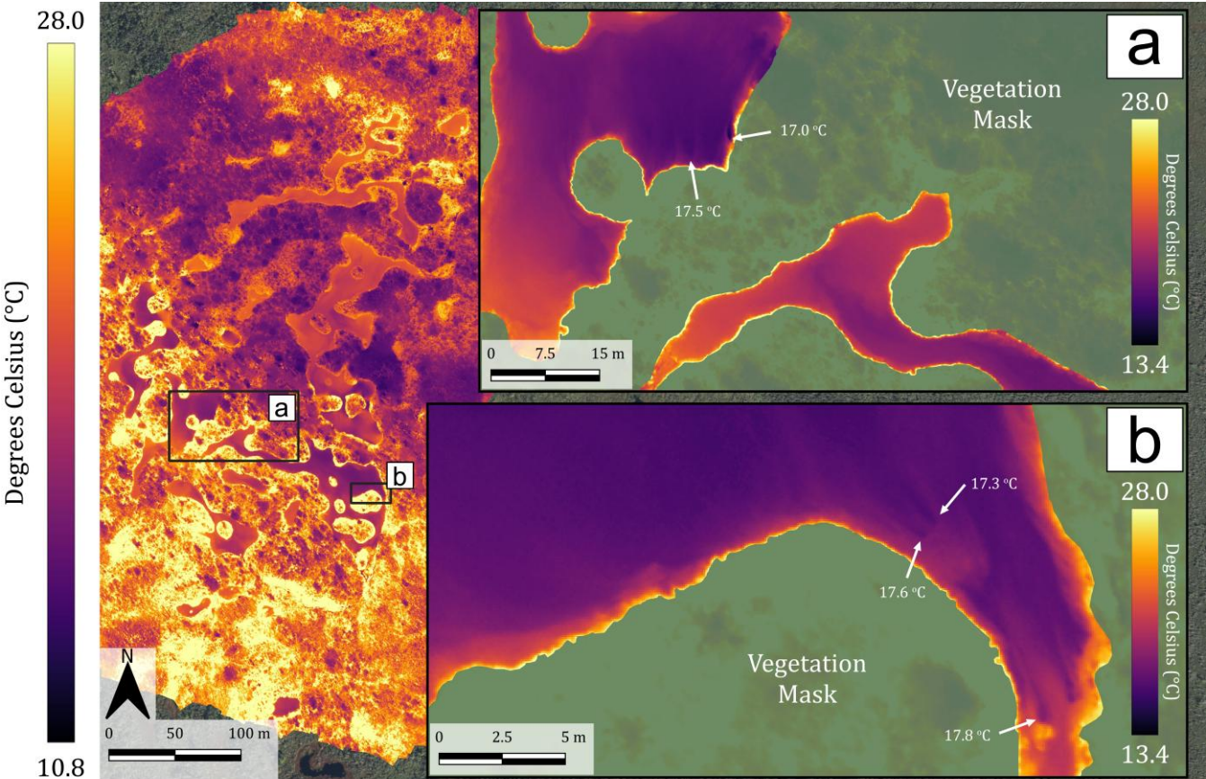
445 Figure 7: Uncrewed aerial system (UAS) Thermal Infrared (TIR) orthomosaic map of Caribou Bog patterned pools captured on June 9 th , 2023, and calibrated against the thermal emissivity of water. Discrete points of cooler water are highlighted in the (a) the
