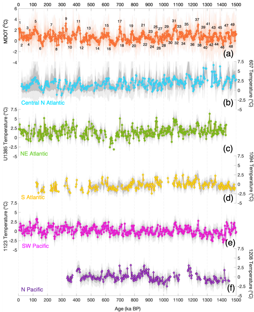
380 Figure 3: Interpolated and bootstrapped Mg/Ca-derived temperature records for all sites. (a) Mean deep ocean temperature stack (MDOT; this study, orange line and markers), with MIS numbers denoting glacial (below) and interglacial (above) stages. Mg/Ca- derived temperature records for: (b) DSDP Site 607 (Ford et al., 2016; Sosdian and Rosenthal, 2009) (light blue); (c) IODP Site 385 U1385 (this study, including additional Iberian Margin records (Birner et al., 2016; Skinner et al., 2003; Skinner and Elderfield, 2007) (light green); (d) ODP Site 1094 (Hasenfratz et al., 2019) (yellow); (e) ODP Site 1123 (Elderfield et al., 2012) (light pink); and (f) ODP Site 1208 (Ford and Raymo, 2020) (dark purple). Mg/Ca-derived temperature records were interpolated on a 3 kyr interval and subsequently bootstrapped. Shading represents 1 and 2\sigma error margins (dark and light grey respectively), propagated from both analytical and calibration sources.
