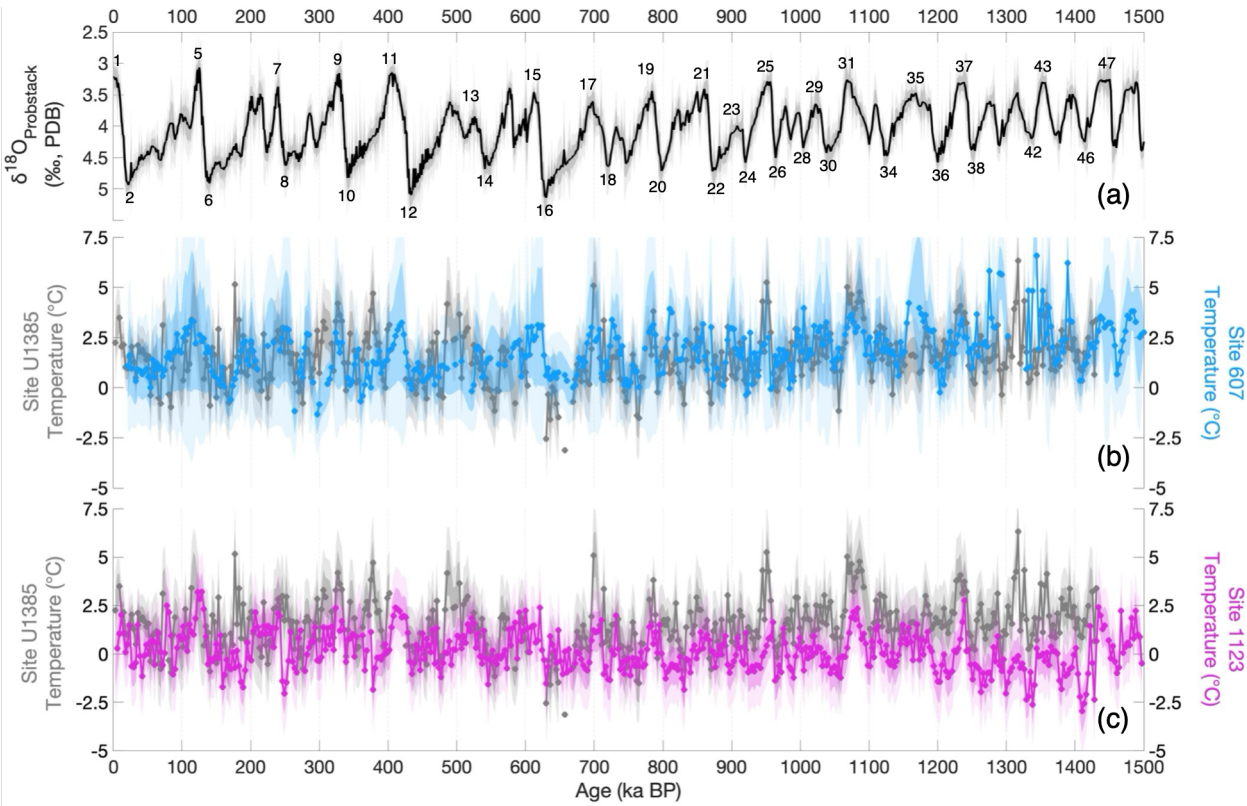
415 Figure 5: Comparison of Mg/Ca-derived deep-water temperature from Site U1385 versus Sites 607 and 1123. (a) Prob-stack benthic \delta^{18}\text{O} (Ahn et al., 2017) (black line), with MIS numbers denoting glacials (below) and interglacials (above). Mg/Ca-derived deep-
