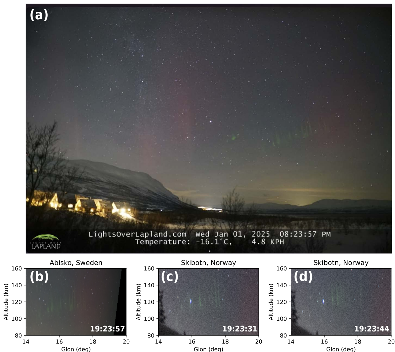
Figure 8. (a) An all-sky image showing a green picket fence structure extending from the center to the right side, accompanied by multiple red auroras. The photograph is reproduced with permission from Lights Over Lapland AB. (b) Projection of panel (a) onto a longitude–altitude plane at a geographic latitude of 71.13^\circ . (c, d) Projections of images captured by the AI camera in Skibotn onto the same plane. Although the images were taken at different times, resulting in slight morphological differences, the overall structures show good agreement. The picket fence was located at altitudes between 110 and 140 km, and the longitudinal separation of each pillar was approximately 5 km.
