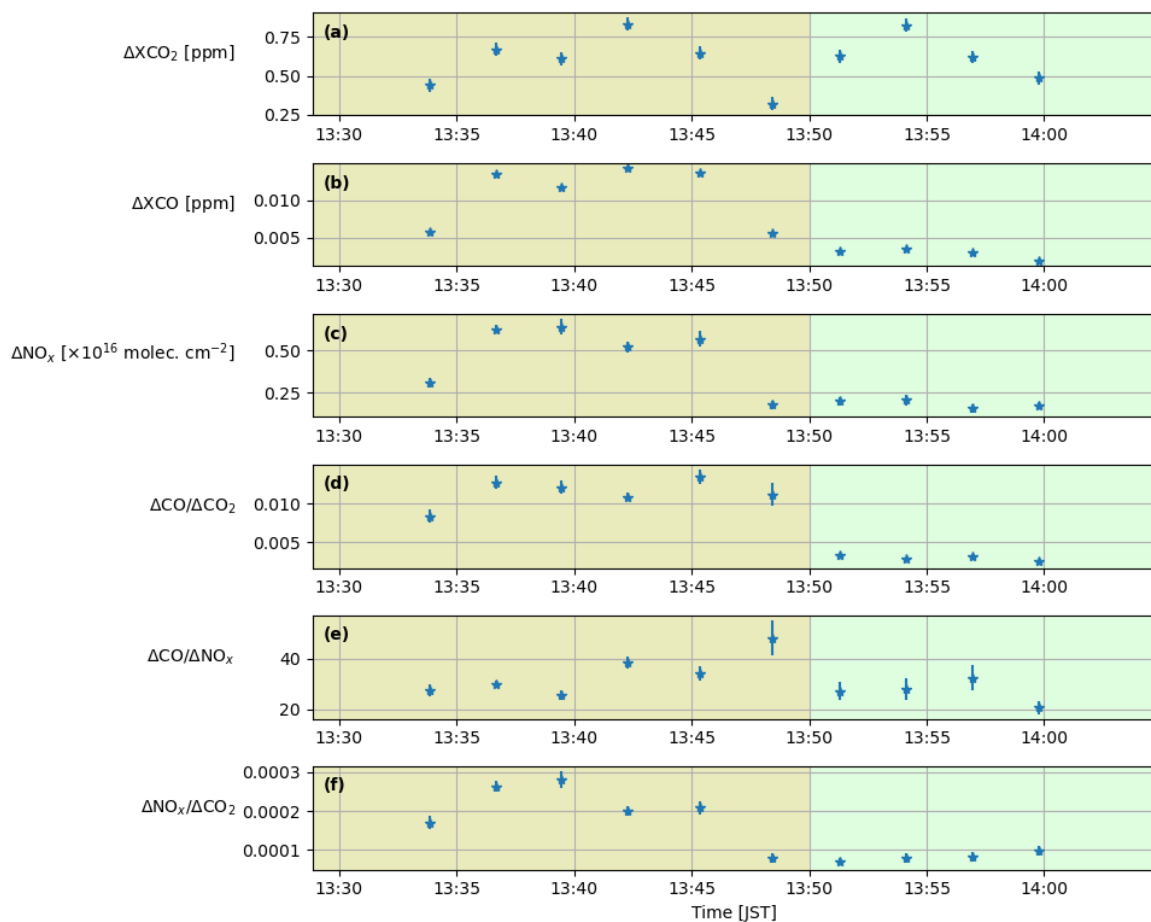
Figure 9. Panels a-c: Enhancements after the subtraction of the background (marked orange in Fig. 8) and trace gas ratios in the plumes measured on 13 November 2023. NO_2 has been converted to NO_x using the conversion factor of 1.32 from Beirle et al. (2019). Panels d-f: Enhancement ratios calculated based on the enhancements shown in panels a-c. The yellow and green background shading refers to episodes A and B as defined in the main text. Error bars in all panels show the respective fit uncertainty from the retrieval and reflect precision only.
