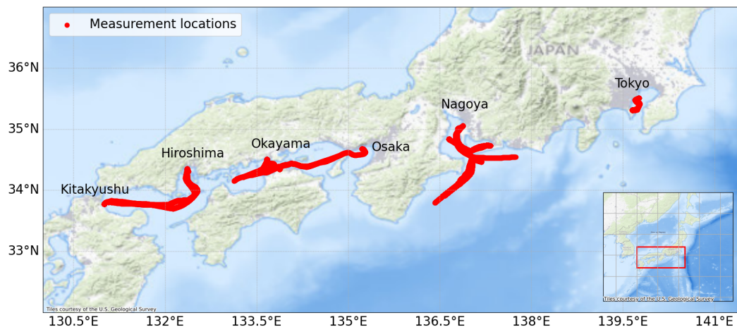
Figure 4. Locations (red) of the columnar measurements collected onboard the vessel Nichiyu Maru between September 2023 and May 2024.
