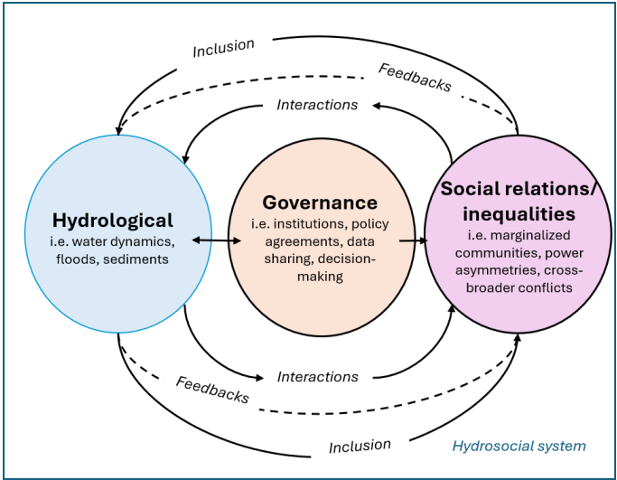
Figure 4: Hydrosocial connectivity conceptualisation
