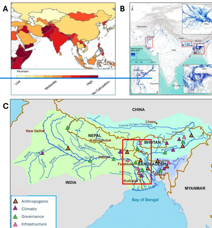
Figure 3: Social vulnerability, flood exposure, and drivers of flood vulnerability in South Asia. The figure overlays the social vulnerability index derived from Burton et al. (2022) with flood exposure/frequency data from Matheswaran et al. (2019) to identify areas where high social vulnerability coincides with substantial flood exposure. Map A (Burton et al. , 2022) shows the social vulnerability index, demonstrating high social vulnerability in South Asia. Map B (Matheswaran et al. , 2019) shows the population exposure to floods. Map C shows the study region. The coloured triangles represent flood hotspot four types—anthropogenic, climatic, governance, and infrastructure-related—each representing distinct yet overlapping drivers of vulnerability, identified through the literature screening (with red box showing area of high flood vulnerability, in a region covering many international borders by screening targeted literatures including 62 publications for full text review). The locations of these markers are intended to provide an illustrative and diagnostic representation of the spatial distribution and interaction of reported drivers rather than a predictive, exhaustive, or quantitatively validated assessment of flood vulnerability and are intended to be illustrative and diagnostic, rather than predictive or comprehensive (see supplementary document for further clarification). The triangles represent flood hotspot four types—anthropogenic, climatic, governance, and infrastructure-related—each representing distinct yet overlapping drivers of vulnerability. The figure was produced by synthesising and overlaying the published source-map information, with generative AI (ChatGPT, OpenAI) used to assist with the graphical rendering and visual presentation of the composite map.
