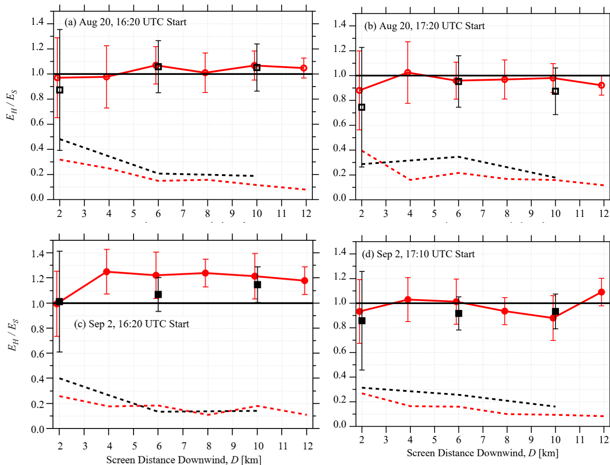
585 Figure 7. As Figure 3 for the flights downwind of the small area sources. Error bars and dashed lines show one standard deviation (calculated from 10 flights).
