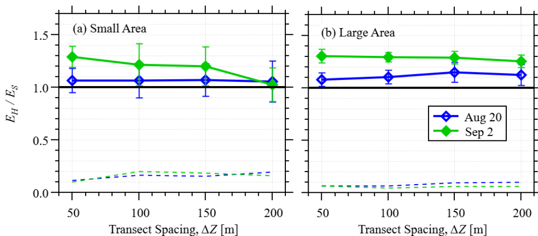
Figure 9. As Figure 6 for the flights downwind of the small (a) and large (b) area sources for the flights starting at 16:20 only. Aug 20 shown as blue, open symbols, and Sep 2 shown as green, closed symbols.
