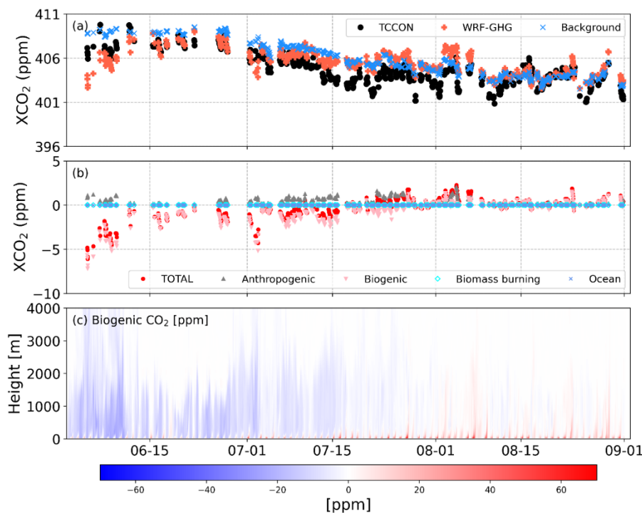
Figure 11. Time series (local time) of (a) observed and simulated total, background, (b) tracer-specific XCO 2 , and (c) variation of simulated biogenic CO 2 mole fractions over time (local time) and height above ground at Orléans/TRN site. The simulated values here are all without AVK smoothing.
