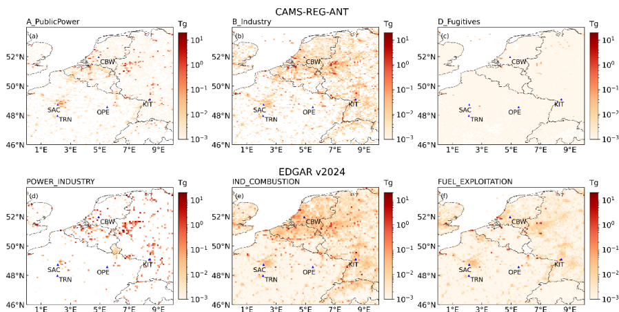
Figure 9. The maps of sector-specific CO 2 emissions for 2018 from CAMS-REG-ANT (a) public power, (b) industry and (c) fugitives sectors, and EDGAR v2024 (d) power industry, (e) industrial combustion and (f) fuel exploitation. All values are shown on a logarithmic scale (base 10, unit: Tg).
