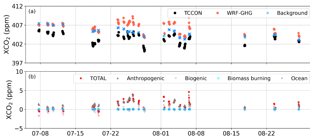
Figure 8. Time series (local time) of (a) observed and simulated total, background, and (b) tracer-specific XCO 2 at Paris site. The simulated values here are all without AVK smoothing.
