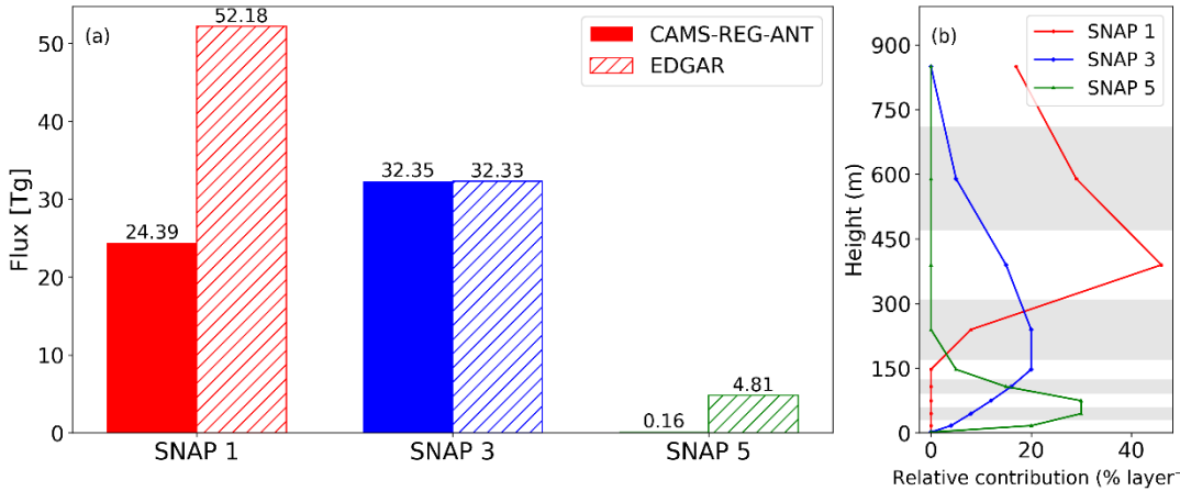
Figure 10. (a) CO 2 emission fluxes from different sectors in 2018 within the area (47.6°N - 50.6°N, 6.94°E - 9.94°E) surrounding the KIT site, and (b) the vertical emission profiles applied for the corresponding sectors, the height refers to the altitude above ground level.
