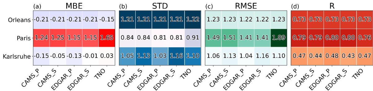
Figure 7. The MBE (a), STD (b), RMSE (c), and R (d) of XCO 2 between five different simulations and observations at three TCCON stations.
