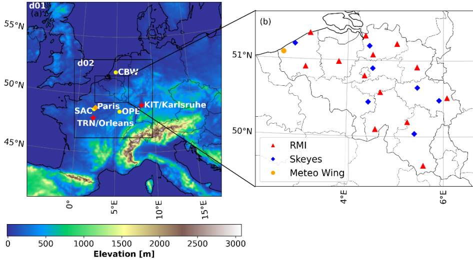
90 Figure 1. Terrain elevation map of the simulated domains, with horizontal resolutions of 9 km (d01) and 3 km (d02), showing ICOS (yellow dots), TCCON (orange diamond) and co-located (red stars) sites within d02 (a), and synoptic stations in Belgium for which data are available for our study period (b).
