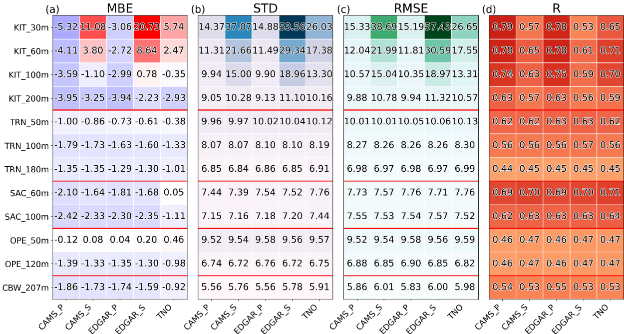
Figure 3. The MBE (a), STD (b), RMSE (c), and R (d) of near surface CO 2 mole fractions between five different simulations and observations at different heights at various ICOS stations. The colors in (a) represent values from negative to positive, with a blue–white–red gradient: negative values in blue, positive values in red, and values near zero in white, whereas in (b–d), more intense colors represent larger values and less intense colors represent smaller values.
