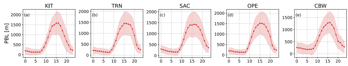
Figure A3. The diurnal cycles (local time) of planetary boundary layer height simulated by WRF-GHG at the KIT (a), the TRN (b), the SAC (c), the OPE (d) and the CBW (e) sites.
