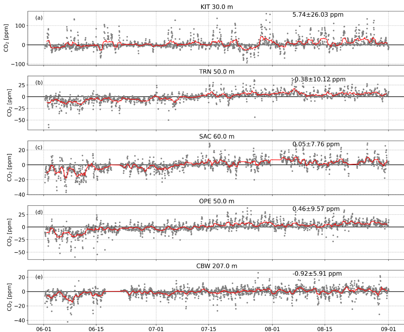
Figure A5. Time series of the between the simulated near surface CO 2 mole fractions using TNO inventory and observed results at 30 m at the KIT (a), 50 m at the TRN (b), 60 m at the SAC (c), 50 m at the OPE (d) and 207 m at the CBW (e) sites, where the values represent the MBE \pm STD between the simulations and observations. The red curve represents the 24-hour moving average.
