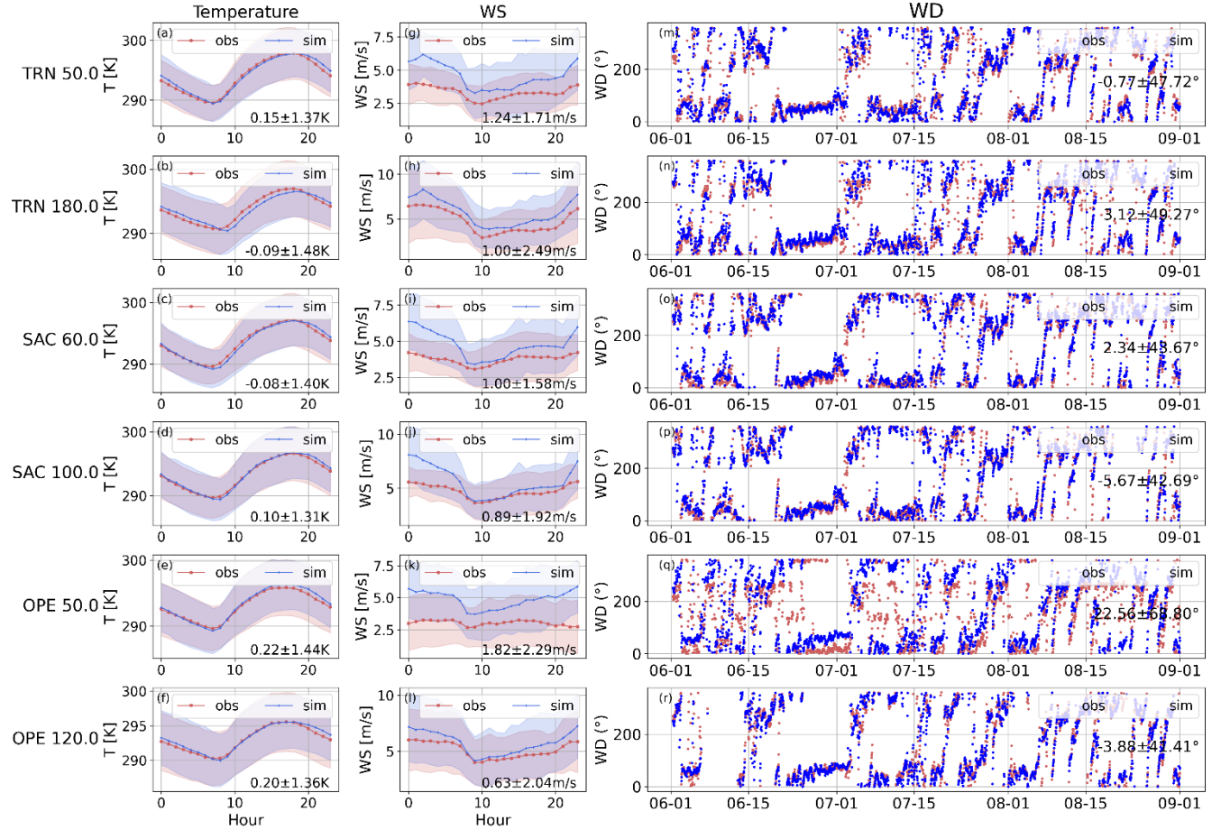
Figure 2. The diurnal cycles of temperature (a-f) and wind speed (g-l), and the time series of wind direction (m-r) at different heights at various ICOS stations. The time is local time (UTC+2).
