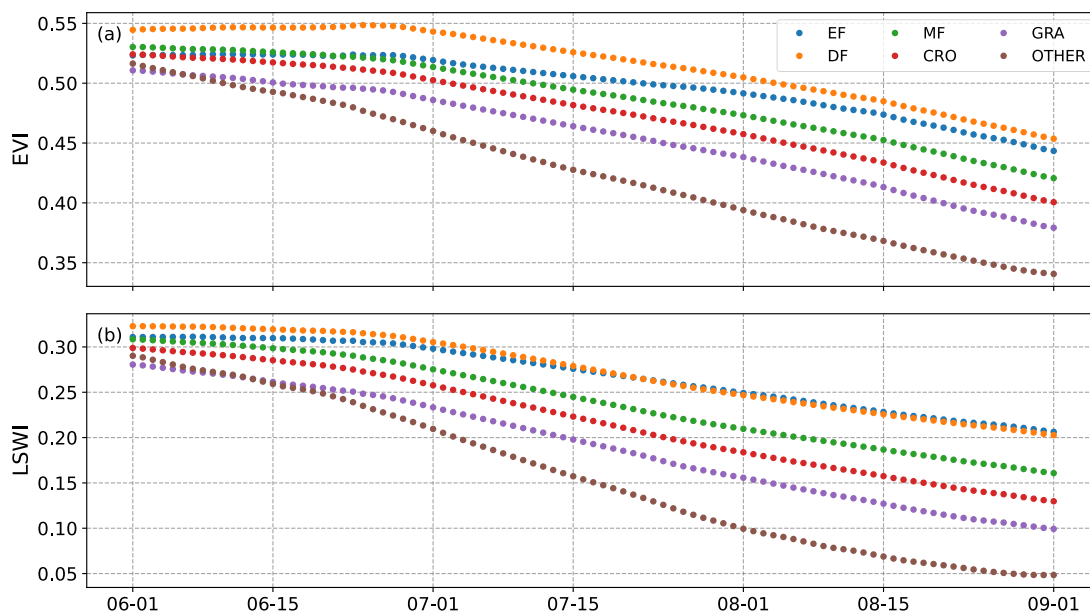
Figure A6. Time series of EVI (a) and LSWI (b) for different vegetation types from MODIS at Orléans/TRN site. According to the land cover data provided by Copernicus, there are no Shrubland (SHR) and Wetlands (WET) vegetation types near Orléans/TRN. Therefore, their corresponding EVI and LSWI values are 0 and are not shown here.
