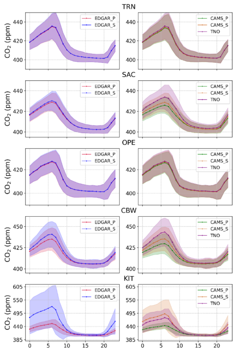
Figure A4. Diurnal cycles (local time) of simulations with different anthropogenic emissions at five ICOS sites at the model lowest layer (approximately 25 m above the ground).
