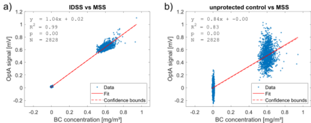
Figure S1: Correlation of the measurements presented in Fig. 4 between the AVL Micro Soot Sensor (MSS) and two optoacoustic (OptA) sensors. The illumination-detection separating sensor (IDSS) is shown on the left, and the unprotected control is shown on the right. The raw signals from the OptA sensors are plotted in mV, while the readouts from the AVL MSS are presented in mg/m 3 . Each graph includes 2828 data points that were taken during the experiment. A line of best fit with confidence bounds is included for each figure. Two groups of points can be distinguished, one roughly at 0 mg/m 3 for the flushing period and one at 0.6-0.7 mg/m 3 during black carbon (BC) measurements. The line of best fit for the IDSS (left) has a R 2 value of 0.99. For the unprotected control sensor (right) the vertical spread of values on both sides of the line of best fit is quite large and the fit has a significantly lower R 2 value of 0.83. These lines of best fit were used to convert the raw signals from both OptA sensors to BC concentrations.
