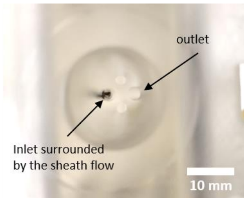
Figure S2: Picture of the ellipsoidal chamber of the optoacoustic illumination-detection separating sensor (IDSS) after the stress test presented in Fig. 3a. The openings for the sample flow (inlet and outlet) are shown. The sample inlet is visibly black, due to deposition of black carbon (BC) particles inside the inlet sensor tube. The rest of the chamber does not show any visible BC particle deposition. This is one more indication that the protective sheath flow effectively limits the diffusion of particles inside the sensor chamber and prevents contamination of sensitive components despite high BC exposure.
