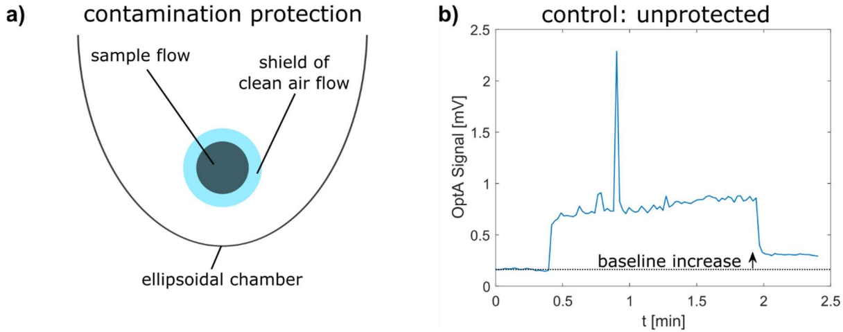
220 Figure 2: Sketch of the sheath flow integrated into the illumination-detection separating sensor (IDSS) that prevents a baseline increase in optoacoustic (OptA) signal. a) Cross-section of the ellipsoid cavity of the IDSS sketched to depict the sheath flow of clean air surrounding the sample flow containing black carbon (BC) particles. b) Representative sample of the OptA signal recorded over 2 min by a control sensor with the sheath flows turned off. The graph shows a clear baseline increase, caused by contamination of the sensor.
