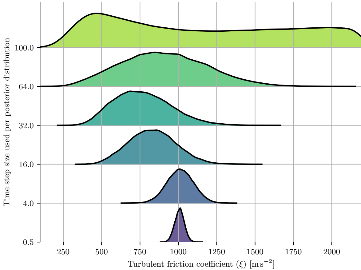
Figure 13. Posterior distributions of turbulent friction coefficient \xi calibrated with a varying temporal resolution of the velocity data. The information gained during calibration increases with temporal resolution.
