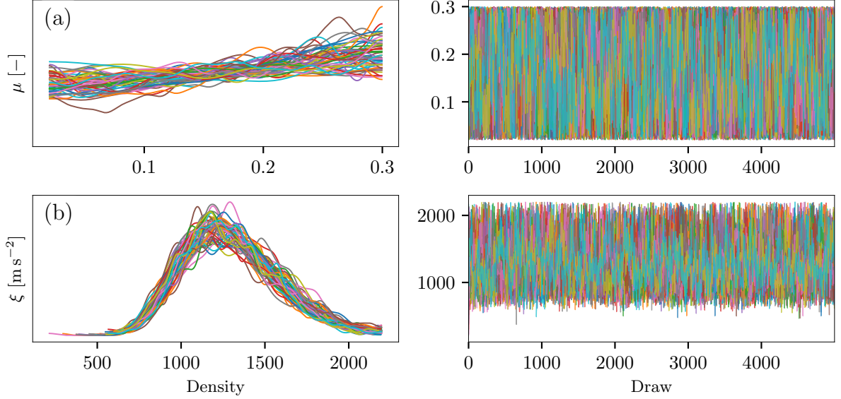
Figure B1. MCMC trace plots for (a) Dry Coulomb friction coefficient ( \mu ) and (b) Turbulent friction coefficient ( \xi ) based on calibration with maximum velocity ( U_{\max} ) as observation. Each color represents an independent chain. Left panels show kernel density estimates of the marginal posterior distributions. Right panels show trace plots across iterations, demonstrating chain convergence and adequate mixing.
