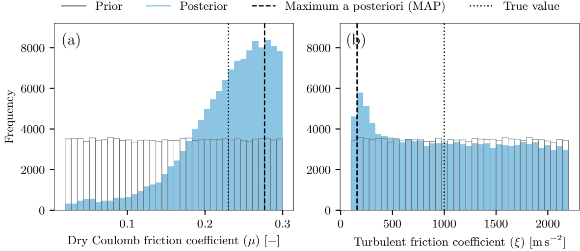
Figure 8. Posterior and prior distributions of (a) Dry Coulomb friction coefficient ( \mu ) and (b) Turbulent friction coefficient ( \xi ) based on a calibration with runout distance ( X_{\text{end}} ) as observation. Greater contraction of the posterior of \mu indicates higher information gain during calibration with the runout distance.
