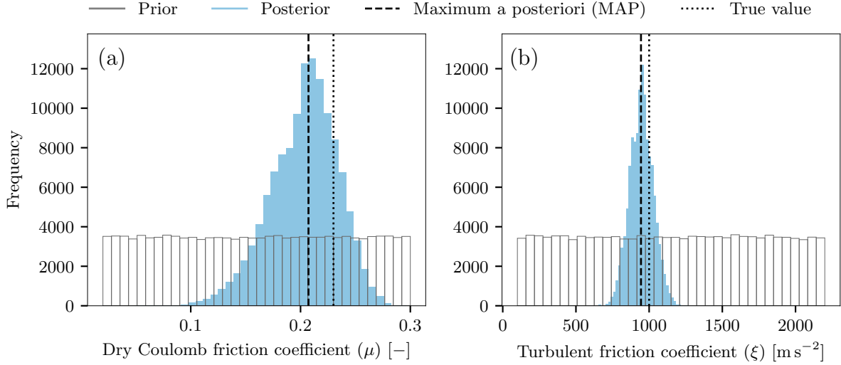
Figure 10. Posterior and prior distributions of (a) Dry Coulomb friction coefficient ( \mu ) and (b) Turbulent friction coefficient ( \xi ) based on calibration with position time series as observation. Similar to velocity time series, position time series also provides information about both parameters, albeit to a lesser extent.
