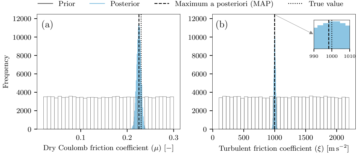
Figure 9. Posterior and prior distributions of (a) Dry Coulomb friction coefficient ( \mu ) and (b) Turbulent friction coefficient ( \xi ) based on a calibration with velocity time series as observation. Velocity time series provides considerably greater information about both \mu and \xi during calibration, as evidenced by the narrower posterior distributions.
