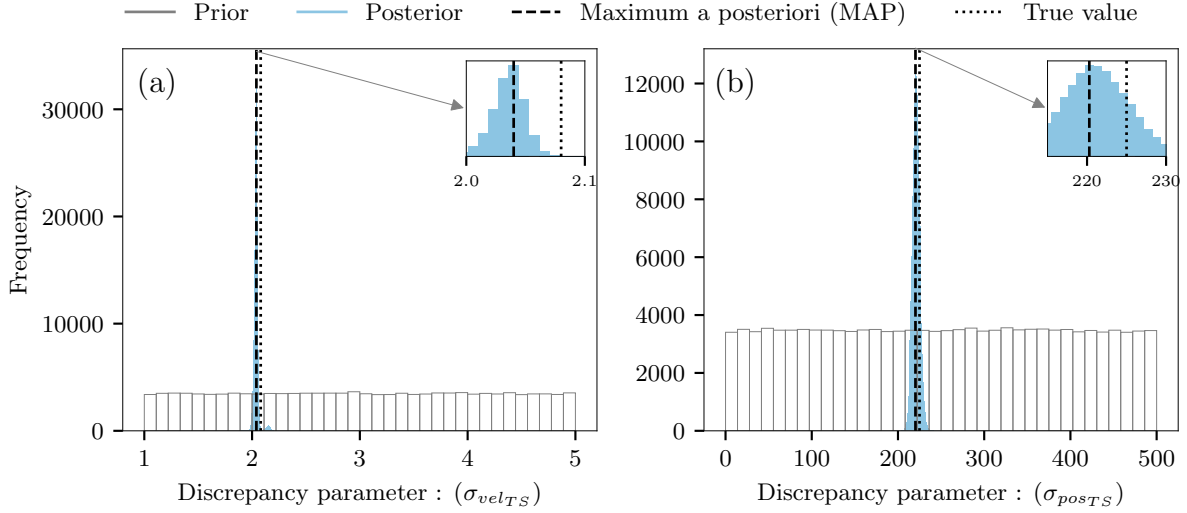
Figure 14. Posterior and prior distributions of (a) Velocity discrepancy parameter ( \sigma_{vel_{TS}} ) and (b) Position discrepancy parameter ( \sigma_{pos_{TS}} ) based on a calibration with velocity and position time series respectively.
