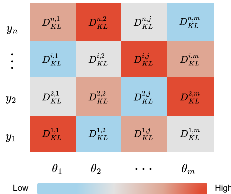
Figure 5. KL divergence matrix generated in the calibration of m parameters with n observation. Each entry of the matrix quantifies the information provided by observation y_i for calibrating parameter \theta_j .
