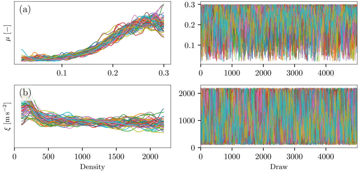
Figure B2. MCMC trace plots for (a) Dry Coulomb friction coefficient ( \mu ) and (b) Turbulent friction coefficient ( \xi ) based on calibration with runout distance ( X_{\text{end}} ) as observation. Each color represents an independent chain. Left panels show kernel density estimates of the marginal posterior distributions. Right panels show trace plots across iterations, demonstrating chain convergence and adequate mixing.
