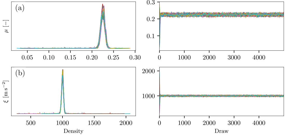
Figure B3. MCMC trace plots for (a) Dry Coulomb friction coefficient ( \mu ) and (b) Turbulent friction coefficient ( \xi ) based on calibration with velocity time series as observation. Each color represents an independent chain. Left panels show kernel density estimates of the marginal posterior distributions. Right panels show trace plots across iterations, demonstrating chain convergence and adequate mixing.
