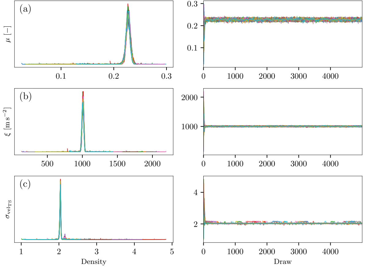
Figure B5. MCMC trace plots for (a) Dry Coulomb friction coefficient ( \mu ) and (b) Turbulent friction coefficient ( \xi ) (c) Velocity discrepancy parameter ( \sigma_{\text{vel}_{\text{TS}}} ) based on calibration with velocity time series as observation. Each color represents an independent chain. Left panels show kernel density estimates of the marginal posterior distributions. Right panels show trace plots across iterations, demonstrating chain convergence and adequate mixing.
