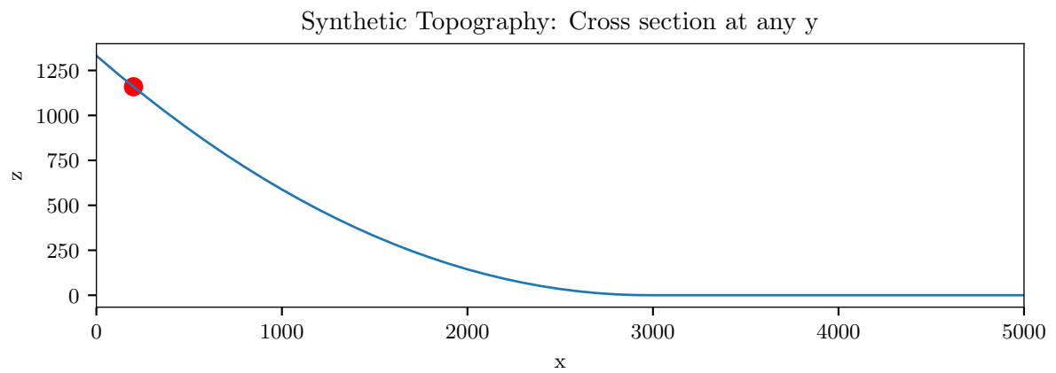
Figure 6. Vertical cross-section of the synthetic topographic model used in this study, with elevation ( z ) plotted against the horizontal coordinate ( x ). The topography is constant along the transverse direction. The red marker denotes the position of the initial release point projected onto this cross-section.
