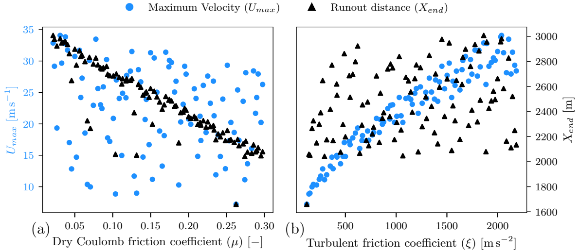
Figure 15. Variation of the friction coefficients ( \mu and \xi ) with maximum velocity ( U_{max} ) and run out distance ( X_{end} ). The dry Coulomb friction coefficient \mu primarily varies with X_{end} , while the turbulent friction coefficient \xi is more strongly influenced by U_{max} .
