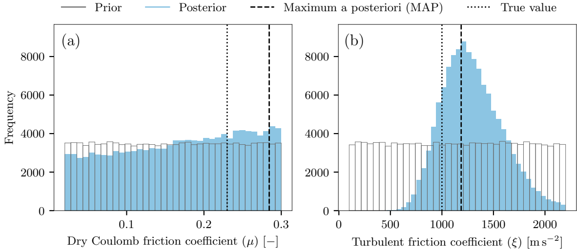
Figure 7. Posterior and prior distributions of (a) Dry Coulomb friction coefficient ( \mu ) and (b) Turbulent friction coefficient ( \xi ) based on calibration with maximum velocity ( U_{\max} ) as observation. Maximum velocity conveyed more information about \xi during calibration, as reflected in the narrower posterior distribution.
