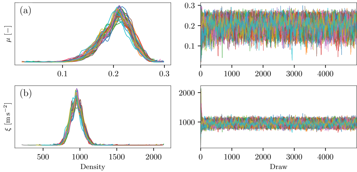
Figure B4. MCMC trace plots for (a) Dry Coulomb friction coefficient ( \mu ) and (b) Turbulent friction coefficient ( \xi ) based on calibration with position time series as observation. Each color represents an independent chain. Left panels show kernel density estimates of the marginal posterior distributions. Right panels show trace plots across iterations, demonstrating chain convergence and adequate mixing.
