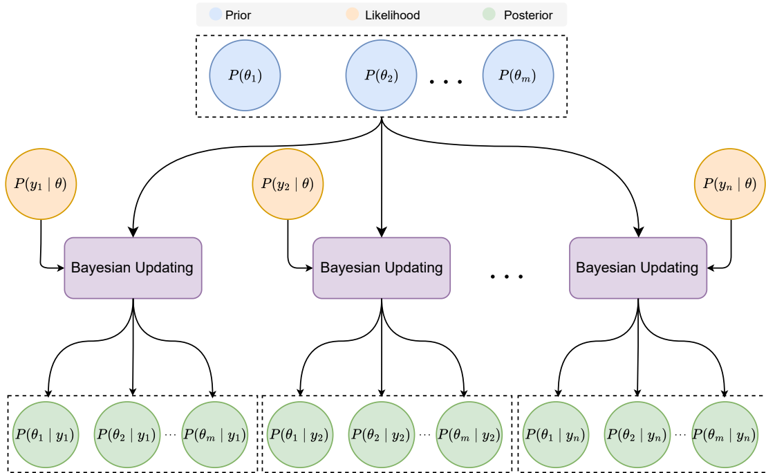
Figure 3. Schematic illustration of the Bayesian data selection process using information-theoretic metrics. Multiple calibration routines are performed in parallel, each using the same likelihood function but leveraging different observations to update the prior distributions. By comparing each resulting posterior distribution against the prior, we can quantify the information gained during calibration relative to observations.
