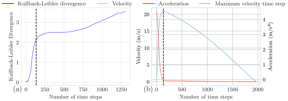
Figure 12. (a) Variation of Kullback–Leibler divergence of the posterior and prior distributions of turbulent friction coefficient \xi with velocity time steps. (b) Variation of velocity and acceleration with time steps.
