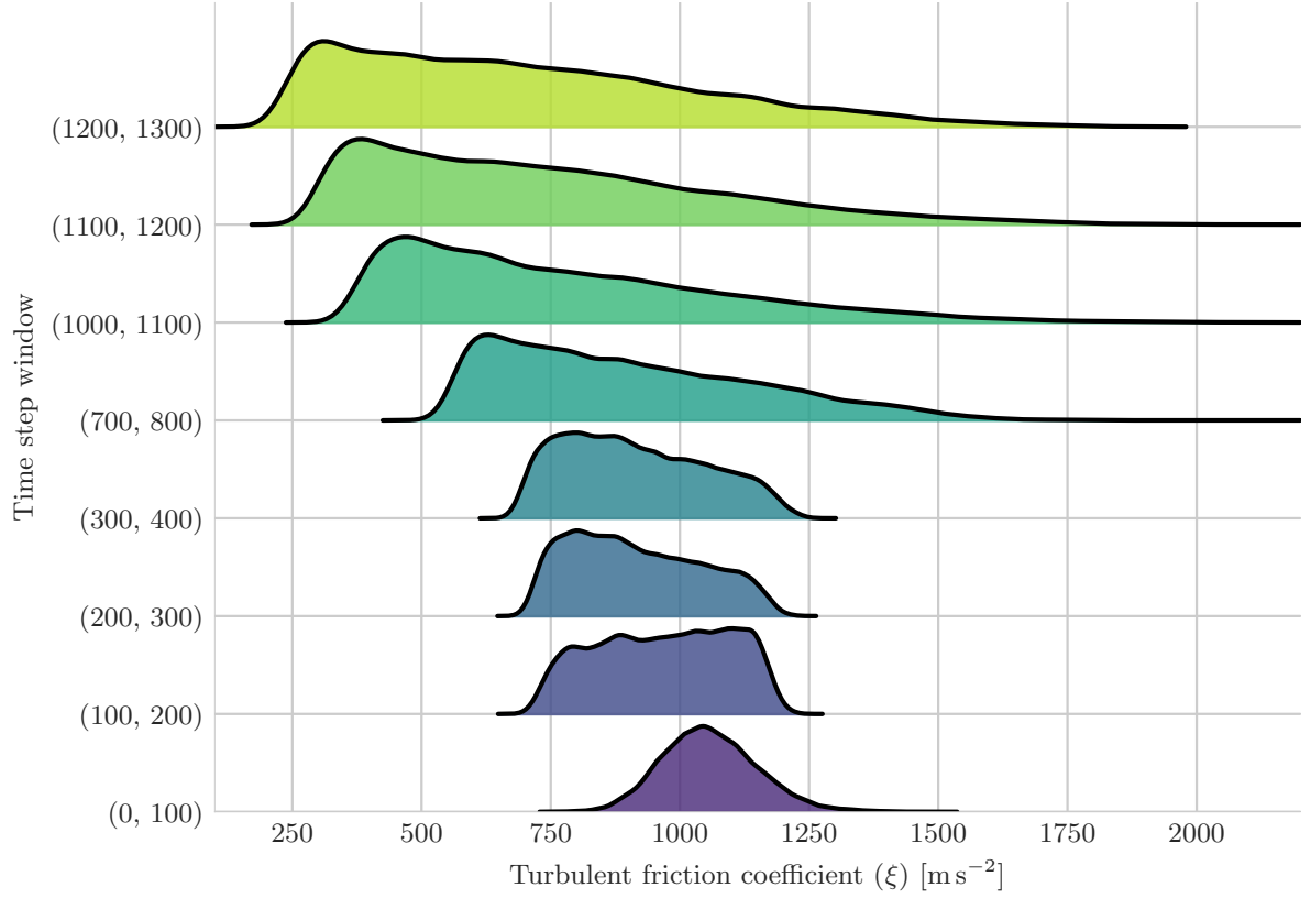
Figure C1. Posterior distributions of turbulent friction coefficient \xi calibrated with a fixed observation window of 100 time steps, with varying onset time. Initial time steps provide the highest information gain.
