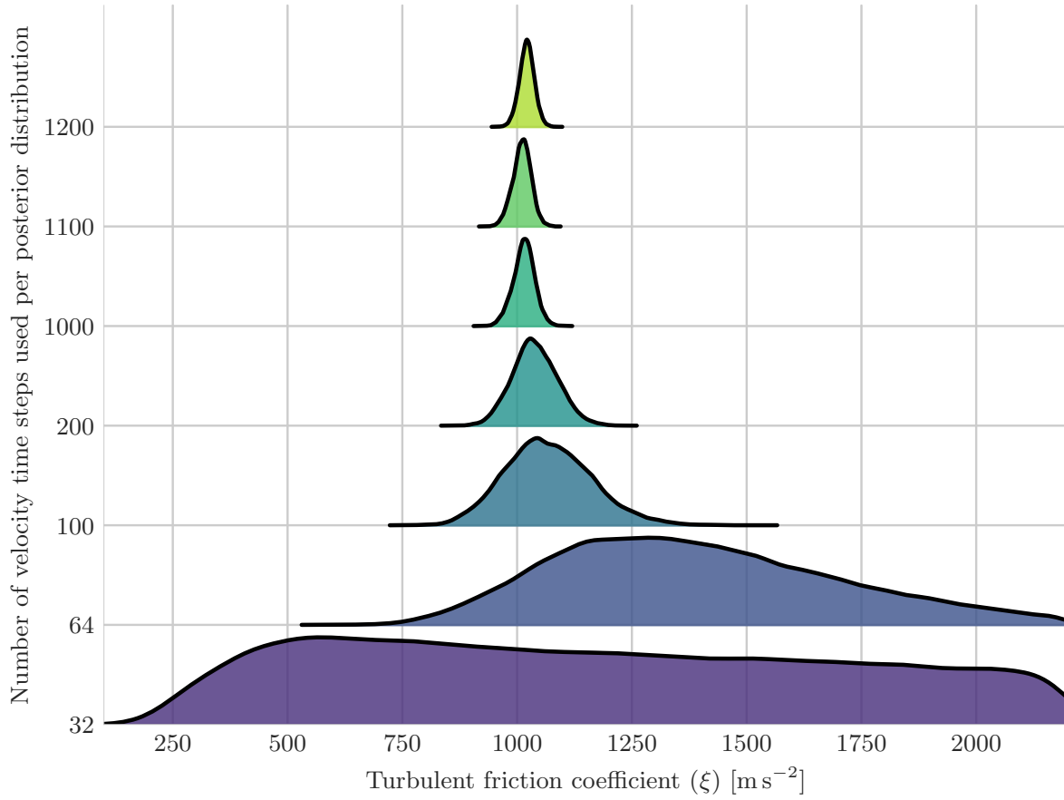
Figure 11. Posterior distributions of turbulent friction coefficient \xi calibrated with a varying number of velocity time steps. The rate of information gain is more profound in the initial time steps than the later.
