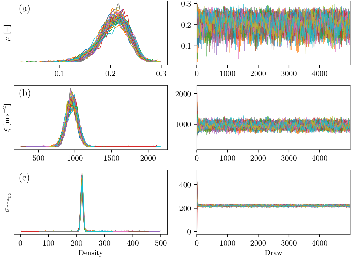
Figure B6. MCMC trace plots for (a) Dry Coulomb friction coefficient ( \mu ) and (b) Turbulent friction coefficient ( \xi ) (c) Position discrepancy parameter ( \sigma_{\text{pos}_{\text{TS}}} ) based on calibration with position time series as observation. Each color represents an independent chain. Left panels show kernel density estimates of the marginal posterior distributions. Right panels show trace plots across iterations, demonstrating chain convergence and adequate mixing.
