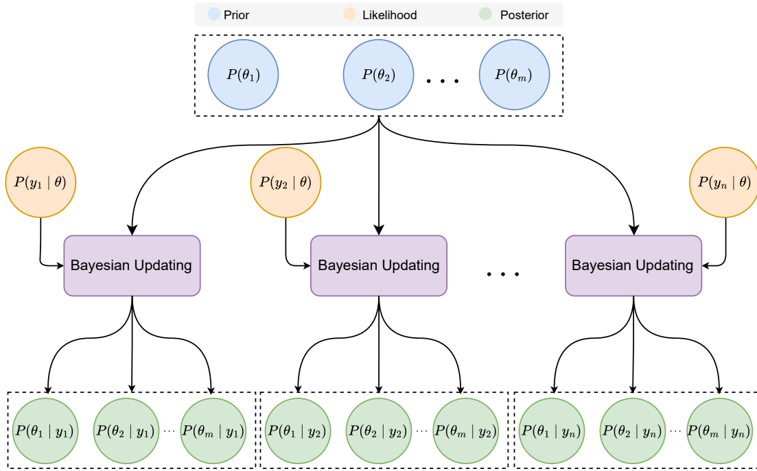
Figure 3. Schematic illustration of the Bayesian data selection process using KL-divergence information-theoretic metrics . Multiple calibration routines are performed in parallel, each using a different the same likelihood function but leveraging different observations to update the prior distributions. These likelihood functions correspond to the available observations and thus by By comparing the each resulting posterior distributions-distribution against the prior distribution- , we can quantify the information gained during calibration relative to observations.
