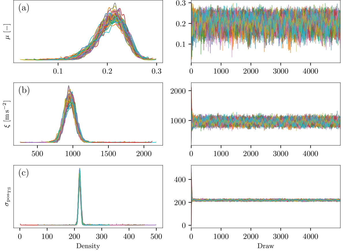
Figure B6. MCMC trace plots for (a) Dry Coulomb friction coefficient ( \mu ) and (b) Turbulent friction coefficient ( \xi ) (c) Position discrepancy parameter ( \sigma_{\text{posrs}} ) based on calibration with position time series as observation. Each color represents an independent chain. Left panels show kernel density estimates of the marginal posterior distributions. Right panels show trace plots across iterations, demonstrating chain convergence and adequate mixing.
