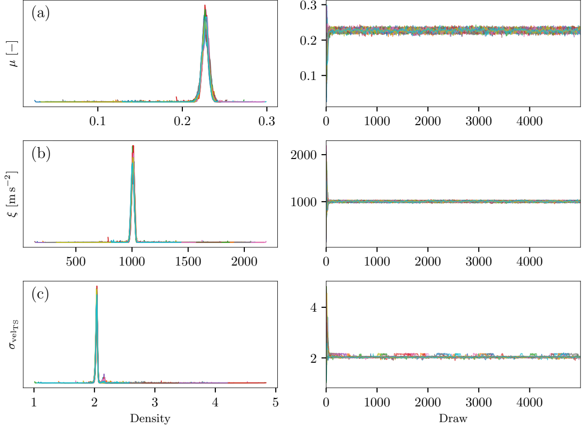
Figure B5. MCMC trace plots for (a) Dry Coulomb friction coefficient ( \mu ) and (b) Turbulent friction coefficient ( \xi ) (c) Velocity discrepancy parameter ( \sigma_{\text{vel}_{TS}} ) based on calibration with velocity time series as observation. Each color represents an independent chain. Left panels show kernel density estimates of the marginal posterior distributions. Right panels show trace plots across iterations, demonstrating chain convergence and adequate mixing.
