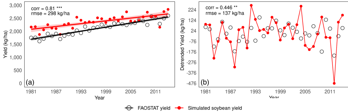
Figure 5. Time-series comparison between simulated yields by MATCRO-Soy and FAOSTAT reported yield data: (a) Global yield and long-term trend during 1981–2014, and (b) Detrended yield during 1981–2014. Correlation for detrended yield was calculated by subtracting linear trend. Symbols ***, **, and * denote p < 0.001 , 0.01, and 0.05, respectively.
