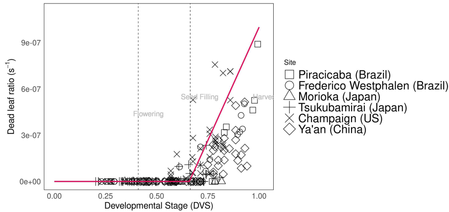
Figure 3. Dead leaf ratio ( \text{s}^{-1} ) during soybean plant development (DVS = 0 – 1). Abbreviations and symbols are the same as in Fig. 2.
