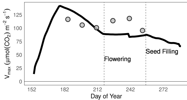
Figure 12. Maximum carboxylation capacity of Rubisco ( \mu\text{mol}(\text{CO}_2)\text{m}^{-2}\text{s}^{-1} ) during the growing period in Cham-paign (US) in 2002 as simulated using MATCRO-Soy (black line) and as measured (grey dots) by Bernacchi et al. (2005).
