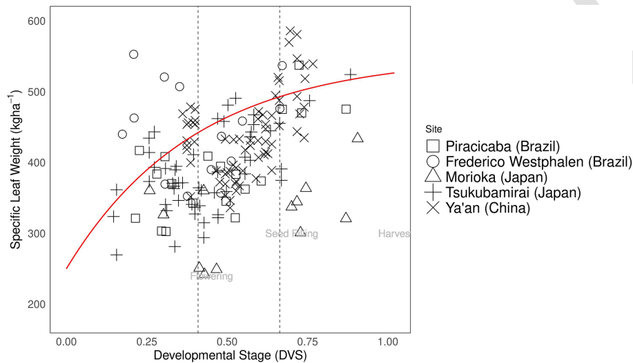
Figure 4. Specific leaf weight ( \text{kg ha}^{-1} ) during soybean plant development (DVS = 0 – 1). Abbreviations and symbols are the same as in Fig. 2.
