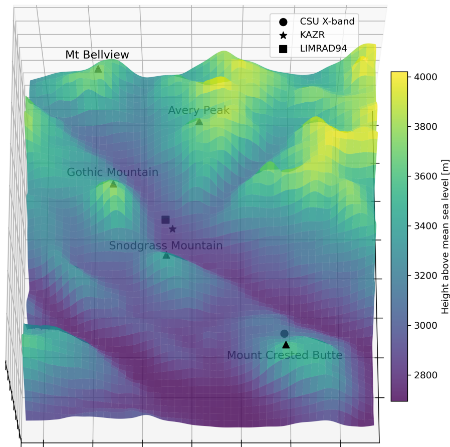
Figure B1. Elevation showing the local topography around the measurement site with all relevant mountain peaks and instrument locations marked. In this view, north corresponds to the top edge of the plot, and east corresponds to the right edge; south and west follow accordingly. Blue and yellow colors mark low and high elevation, respectively.
