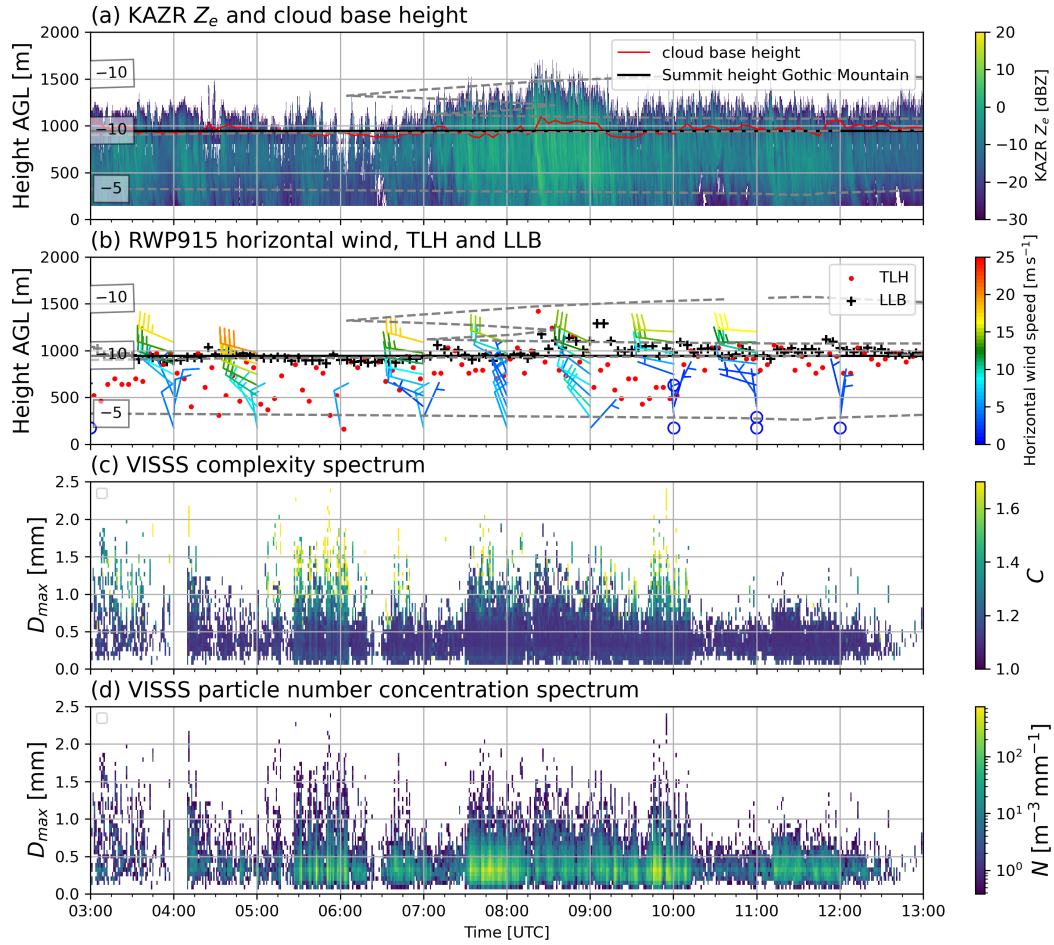
Figure 3. Case study on Feb. 21 2023. (a) KAZR Z_e and ceilometer cloud base height (solid red line) with the summit height of Gothic Mountain (black) overlaid. Grey dashed lines are the isotherms with respective labels on the left. (b) RWP915 horizontal wind barbs (color shading) with turbulent layer height (TLH, red dots) and liquid layer base height (LLB, black crosses). (c) VISSS complexity spectrum as a function of maximum particle diameter ( D_{max} ). (d) VISSS particle number concentration spectrum as a function of D_{max} .
