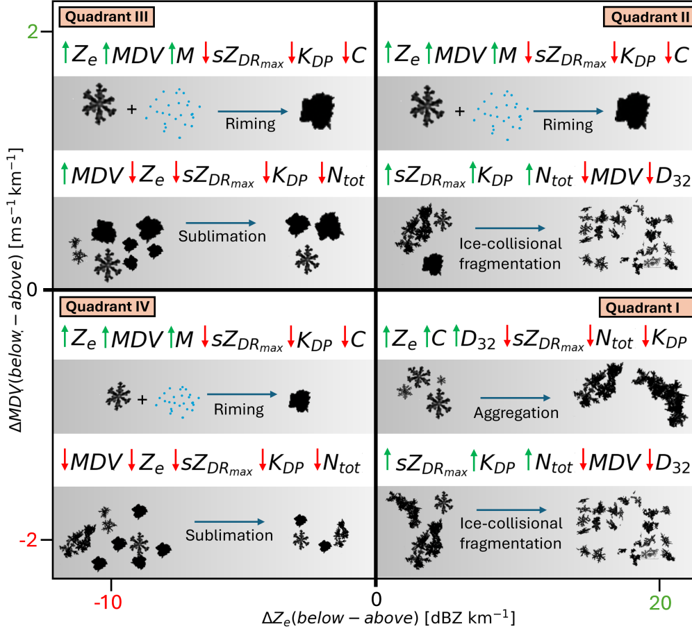
Figure 12. Conceptual diagram of the suspected (dominant) microphysical processes inside the turbulent layer, displayed similar to the four quadrants in Fig. 11. The impact of microphysical processes on radar and VISSS variables is also displayed qualitatively: Red downward facing arrows indicate a decrease of the respective variable, upward facing green arrows an increase. Note that for the radar variables ( Z_e , MDV , sZ_{DR_{max}} and K_{DP} ), we can measure the change inside the turbulent layer. VISSS variables ( N_{tot} , C , D_{32} , M ) are measured below the turbulent layer. Their change due to the microphysical process is suspected based on the change of particle and PSD properties. If a variable is not depicted, no clear trend can be derived. The shown particle images were recorded by VISSS.
