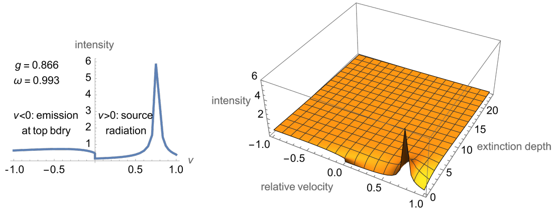
Figure 1. Intensities for strongly forward scattering media: (left) emission ( v < 0 ) and source ( v > 0 ) radiation. (right) internal intensities. v > 0 shows particles descending deeper into the media at the different relative velocities, v < 0 are light particles ascending towards the top.
