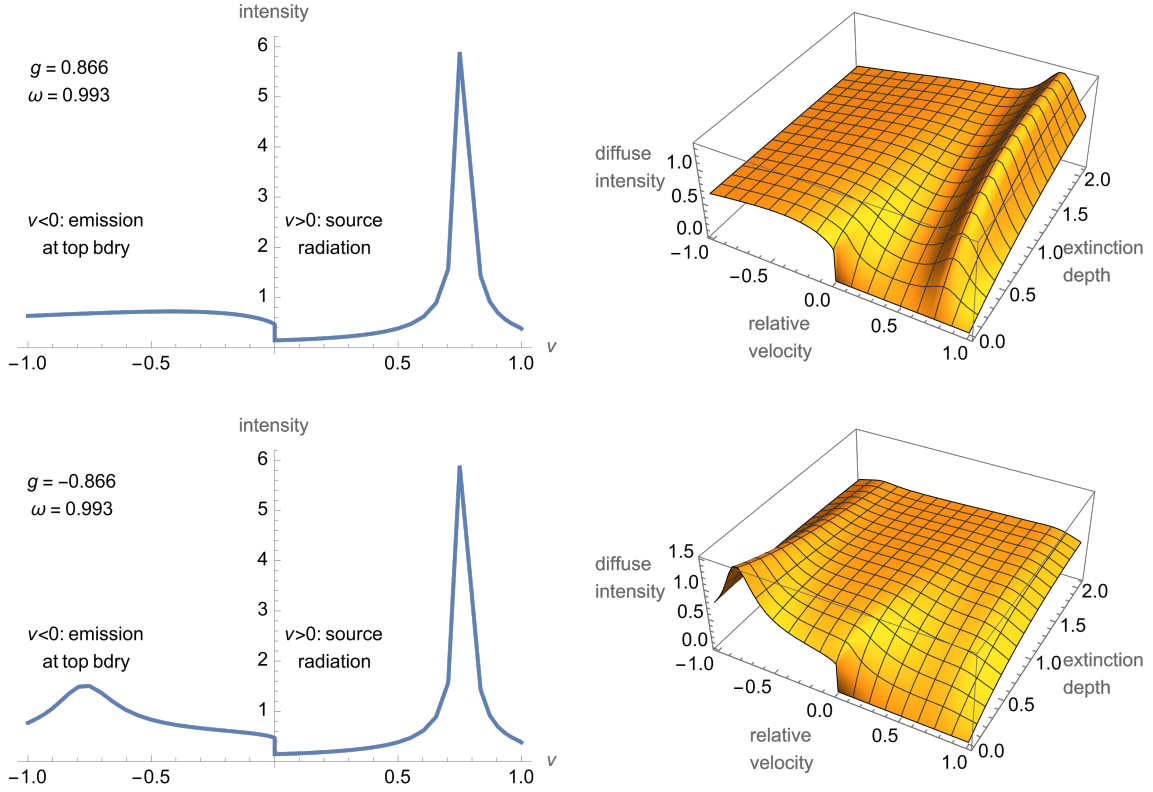
Figure 3. Internal diffuse intensities: (top) strongly forward scattering media, showing a diffuse emission and a strong internal peak at the source peak; (bottom) strongly backscattering media, showing a emission peak at the source peak, and a diffuse internal intensity.
