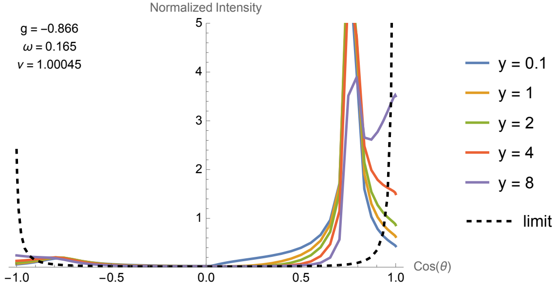
Figure 8. Asymptotic radiance distribution as depth y increases for a high absorption media ( \omega = 0.165 ). The direct source intensity (the peak at the right) dominates the diffuse limit.
