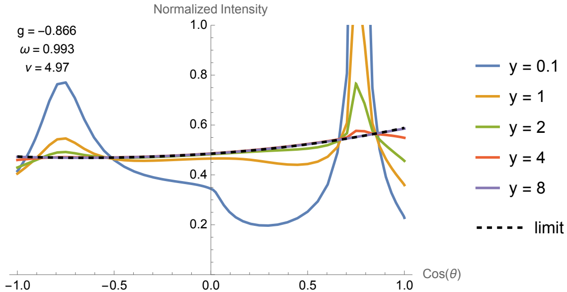
Figure 7. Asymptotic radiance distribution for a low absorption media ( \omega = 0.993 ). As depth y increases, the diffuse internal intensity dominates the direct source intensity (the peak at the right) and the normalized intensity converges to the diffusion limit.
