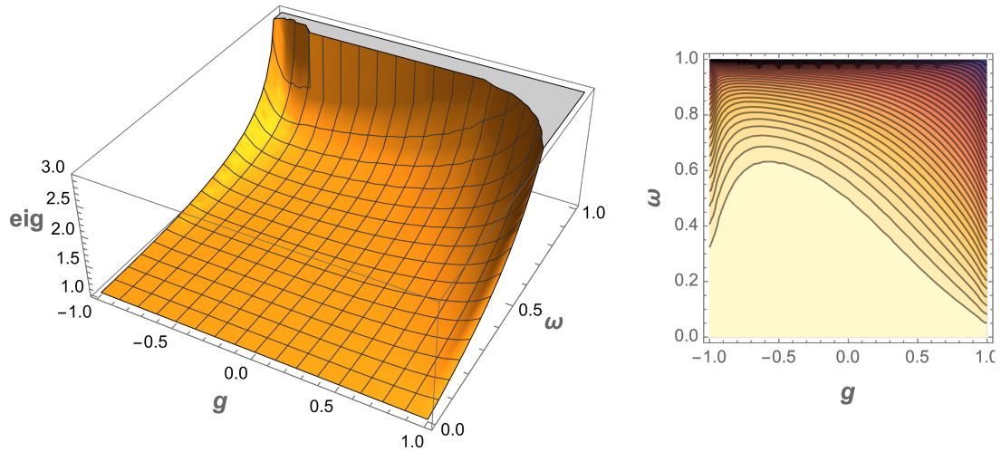
Figure 6. Maximum eigenvalues for varying asymmetry g and scatter fraction \omega . The maximums increase as \omega increases, i.e. as absorption decreases.
