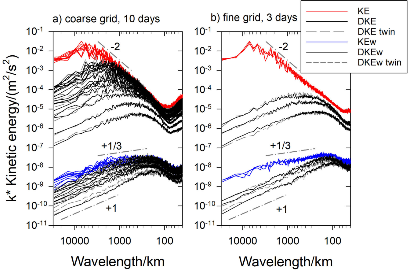
655 Figure 17. Spectra of kinetic energy multiplied with wavenumber k , k = 2 \pi/\text{wavelength} , of horizontal velocities (KE) and of vertical velocity (KEw) from ICON and corresponding spectra (DKE and DKEw) of the velocity differences between the ICON-CoCiP 1-way and 2-way runs, a) for 10-day forecasts on the coarse grid, b) for 3-day forecast on the fine grid, both starting 0 UTC 25 June 2021. The curves show 24-h mean values at subsequent days. For KE and Kew, the curves fluctuate irregularly from day to day. For DKE and DKEw, the values grow with time from day to day. Straight dash-dotted lines indicate the -2 and +1 and 1/3 power-law slopes. The grey dashed lines shown for DKE and DKEw spectra show the results of the twin experiment. The twin results for KE and KEw are not plotted, since they are virtually undistinguishable from the (red and blue colored) contrail results. 660
