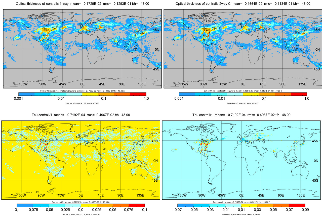
Figure 10. Solar optical depth of contrails on average over hours 24 to 48 after initiation at 0 UTC 25 June 2021. Top left panel: 1-way mode, top right: 2-way mode, bottom: difference. The top panels are color coded in logarithmic scales; the bottom in linear scales, with two different color scaling: the left emphasizes small variations near zero, the right shows optical depth variations exceeding \pm 0.01 . Plots generated from coarse grid simulations
