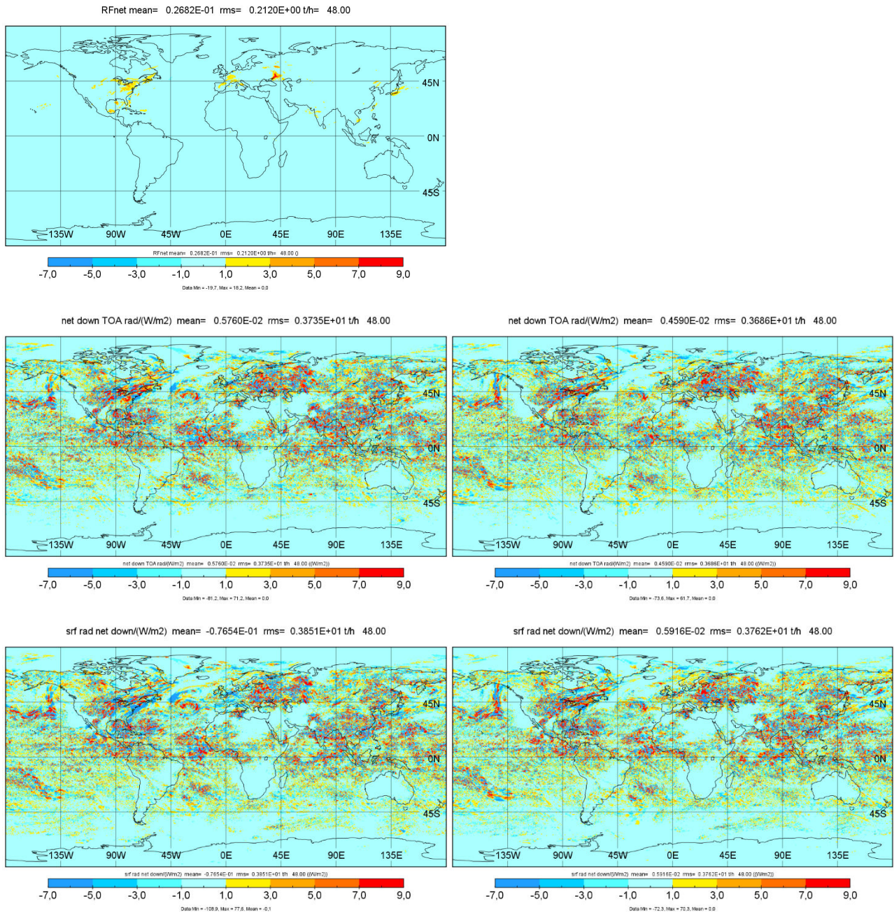
Figure 11. Radiative forcing in \text{W/m}^2 , on average over day 2 after initiation at 0 UTC 25 June 2021 (coarse grid). Top: CoCiP RF model. Middle: net downward radiation difference between 2-way and 1-way mode computed with ecRad in ICON, at TOA. Bottom: same as middle for BOA (surface). The left panels show the effects of contrails. The right panels show the same but from the twin experiment with random instead of contrail forcing. Note that the color scales selected do not include the extreme values of order 80 \text{ W/m}^2 and are insensitive to noise within \pm 1 \text{ W/m}^2 .
