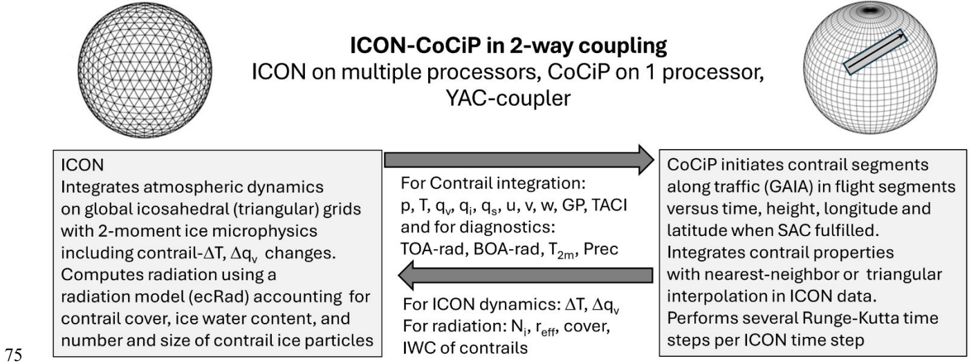
75 Figure 1. ICON-CoCiP coupling concept. From ICON: p : pressure (in Pa); T : temperature (K); q_v , q_i , q_s : mass fractions of water vapor, ice and snow (kg/kg); u , v , w : wind velocities (easterly, northerly, and upward, in m/s); GP : geopotential ( m^2/s^2 ), TACI = \tau_{cirrus} : solar optical depth of cirrus clouds above given height (1); TOA-rad , BOA-rad : top of atmosphere and bottom of atmosphere (surface) downward radiation fluxes ( W/m^2 ); T_{2m} : temperature at 2 m height above ground (K); Prec : total precipitation amount at the surface (m). From CoCiP: \Delta T , \Delta q_v : temperature and humidity changes by contrails (K and kg/kg), N_i : number of ice particles in the contrail (1/kg), r_{eff} : effective contrail ice particle radius (m), cover (m 2 /m 2 ), IWC : contrail ice water content (kg/kg).
