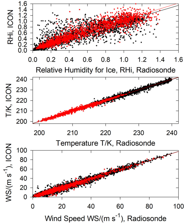
250 Figure 2. Correlations between Radiosonde observation data and ICON-2-way model results on fine grid for relative humidity with respect to ice (RHi), temperature (T), and windspeed (WS). Black symbols: for all conditions between 120 and 500 hPa (about 5.6 to 17 km) height. Red symbols: for conditions when the SAC is satisfied. For correlation statistics see Table 1 . The red correlation line in the top panel indicates that the ICON RHi values are about 5% higher than the radiosonde data in the analysis for SAC satisfied. .
