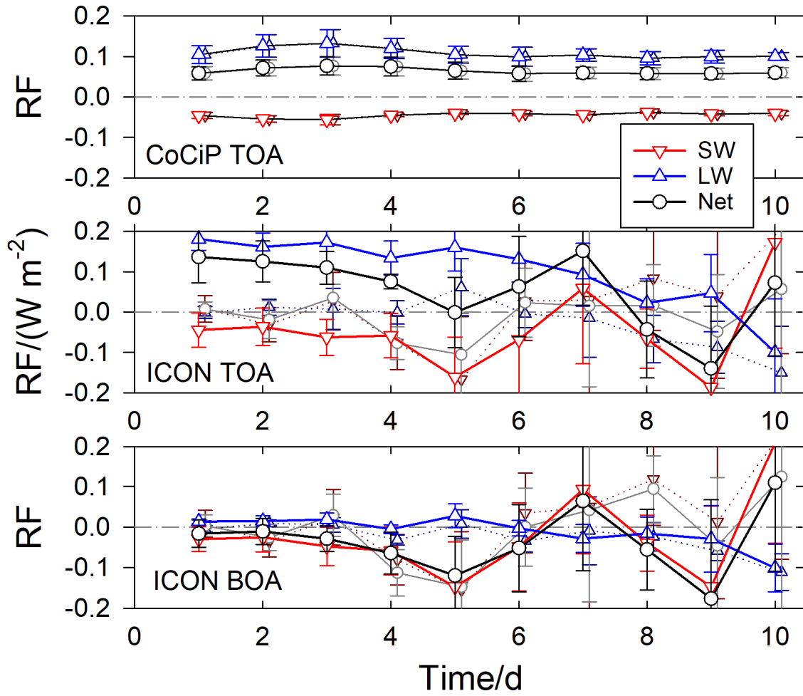
Figure 14. Daily mean RF values (all in W/m^2 ), showing the contrail induced SW RF in red (triangles down), the LW RF in blue (triangles up), and the net value in black (circles) on average over the four test days in 2021 versus forecast time. The errors bars indicating rms values from the 4 simulations. The dotted curves are the results of the twin experiment. They are plotted with temporally slightly shifted error bars. The top panel shows the RF as computed with CoCiP for given atmosphere and contrail properties. The second panel shows the RF as derived from the differences between the downward TOA fluxes in the ICON runs with and without contrail feedback. The lower panel shows the same for the surface fluxes. Note the correlation between ICON TOA and ICON BOA RF values for later days
