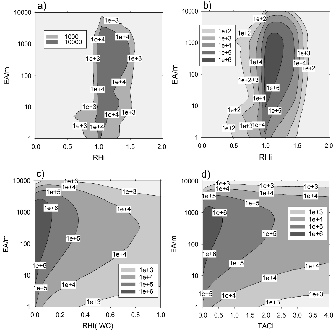
390 Figure 6. Occurrence number of contrails with optically effective cross-section area EA' , with EA' = \tau W \exp(-0.2 \tau_{\text{cirrus}}) , counted in the sum over four 48-h-simulations starting in four days in 2021 as before. Here \tau is the solar optical thickness of the contrail, W is the contrail width and \tau_{\text{cirrus}} is the solar optical depth of cirrus above the contrail. The panels show the occurrence numbers a) for freshly formed contrails versus relative humidity over ice (RHi) in the ambient air, and b-d) for ageing contrails versus b) ambient RHi, c) ambient cirrus ice water content converted to relative humidity RHi(IWC), and d) 395 total solar optical thickness \tau_{\text{cirrus}} of ambient cirrus (TACI) between TOA and 500 hPa.
