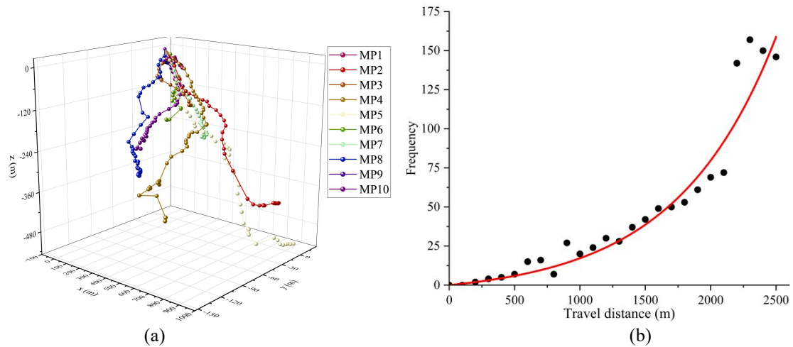
Fig10. (a) movement trails of 10 monitoring points and (b) the plot of travel distance vs. collision frequency.
