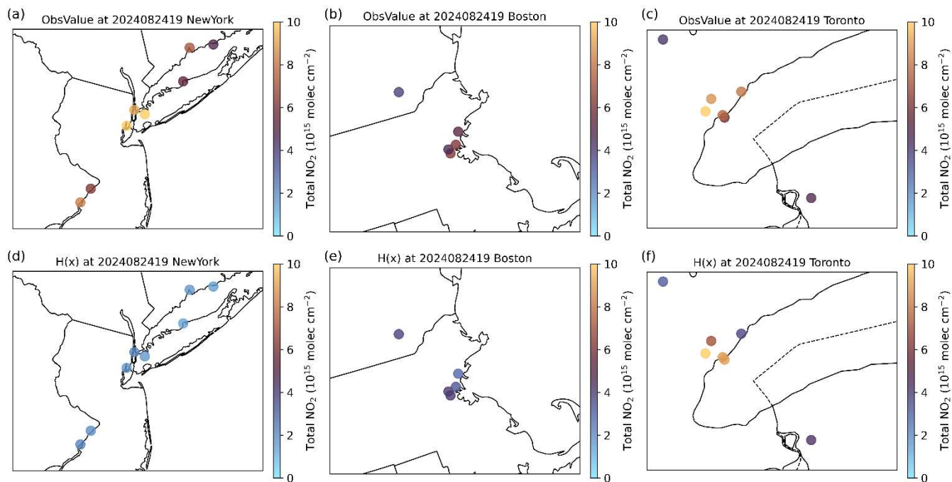
Figure 4. Spatial distribution of PANDORA total column \text{NO}_2 retrieval observations and H(x) over (a, d) New York, (b, e) Boston, and (c, f) Toronto areas valid between 13:30 and 14:30 LST (18:30 and 19:30 UTC) 24 August 2024. H(x) is based on the 19-hour forecast valid at 14:00 LST (19:00 UTC 24) August 2024 from WRF-Chem.
