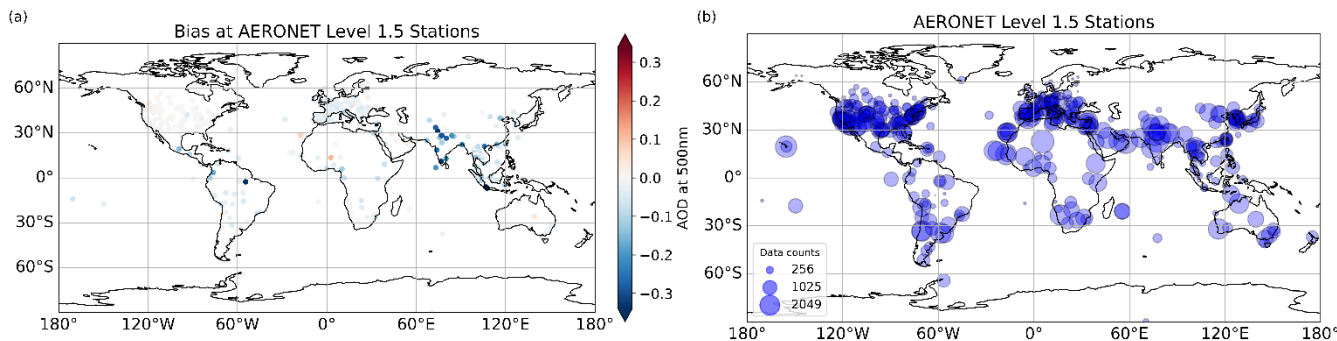
425 Figure 8. (a) Mean bias and (b) data volume of AERONET Level 1.5 stations for November 2024.
