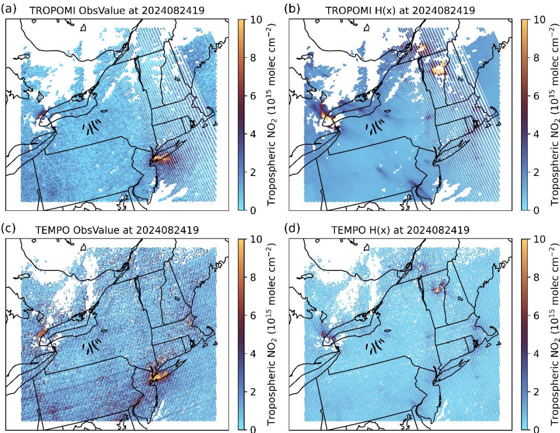
325 Figure 2. Spatial distribution of tropospheric NO 2 retrievals from (a) TROPOMI ObsValue and (b) TROPOMI H(x) and (c) TEMPO ObsValue and (d) TEMPO H(x) valid between 13:30 and 14:30 LST (18:30 and 19:30 UTC) 24 August 2024. H(x) is based on the 19-hour forecast valid at 14:00 LST (19:00 UTC) 24 August 2024 from WRF-Chem.
