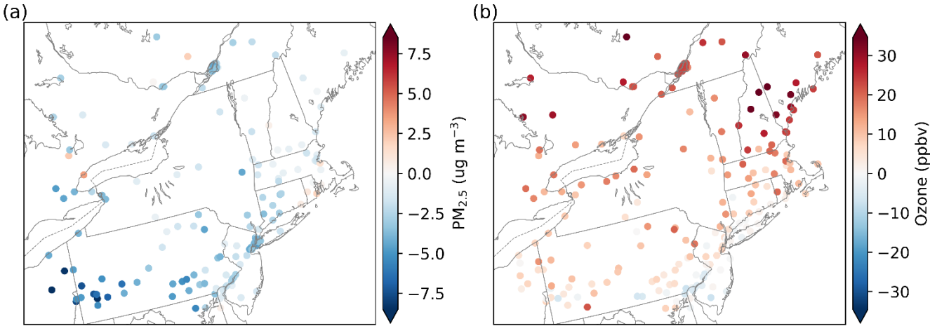
380 Figure 5. Mean bias of WRF-Chem simulations of (a) PM 2.5 and (b) ozone against AirNow sites from 22 August to 1 September 2024.
