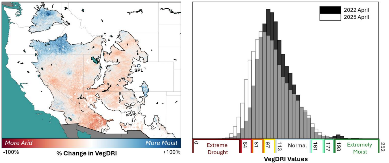
Figure A2: Surface map of percentage change in aridity of April 2025 as compared to 2022 of North American desert regions as indicated by the Vegetation Drought Response Index (VegDRI) (panel a) and distribution of extreme drought and extreme moist conditions during April 2022 and 2025 (panel b); VegDRI values presented in panel b correspond to aridity values in Figs. 7 and A3. The VegDRI was retrieved and averaged over April 2022 and April 2025 separately. Differences between dry and moist conditions between these two months were calculated as percentage differences: 100\% \times (\text{avg}_{2025} - \text{avg}_{2022}) / (\text{avg}_{2022}) .
