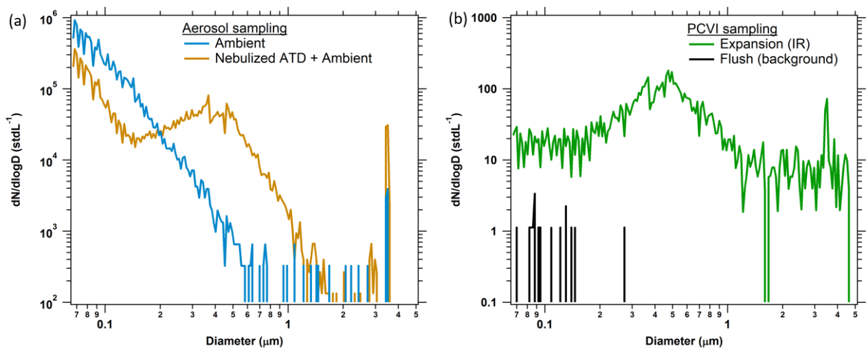
Figure 2: Size distributions measured during a PCVI diagnostic experiment at SPL at a temperature of -29 \text{ }^\circ\text{C} determined with the SPX. (Panel a) The size distribution of ambient aerosol compared to a mixture of ambient aerosol with a nebulized ATD solution (plus a dilution flow) clearly shows the presence of larger aerosol particles when ATD is present. (Panel b) The size distribution determined downstream of the PCVI while PINE was in the flush mode (black line) and in the expansion mode (green line) sampling the ambient/dust mixture. Size distributions are the average of 47 PINE experiments. Above a size of 0.45 \mu\text{m} a clear reduction of particles in the flush (background) is observed. The ice residual concentrations during expansions of 31.9 and 29.7 \text{ stdL}^{-1} (small particles below 0.45 \mu\text{m} , large particles above 0.45 \mu\text{m} ) were higher than the background concentrations during the flush mode of 0.18 and 0 \text{ stdL}^{-1} by a factor of 180 and more than 2560, respectively (lower limit). Concentrations in panel b are down-scaled by the PCVI concentrating factor of 31.8.
