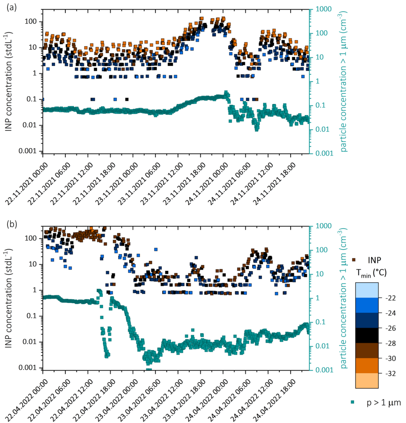
Figure 8: Timeseries of the INP concentration and aerosol particle concentration larger than 1 μm from November 22 nd to 24 th 2021 (panel a) and from April 22 nd to 24 th 2022 (panel b). Blue and brown colors present the nucleation temperature ( \pm 1 °C), and green the aerosol particle concentration larger than 1 μm. INP concentrations below the LOD are presented as values of 0.1 stdL -1 .
