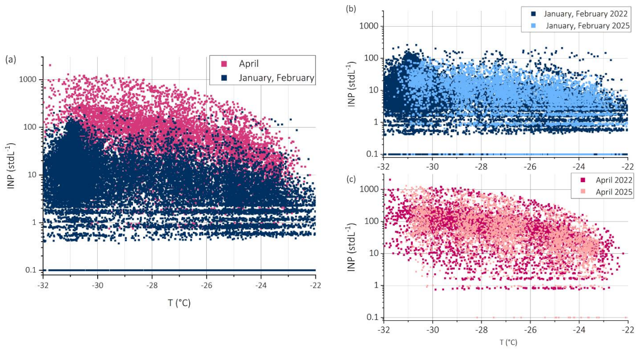
Figure 5: INP concentration as a function of temperature for the measurements in April and January, February from both measurement campaigns in 2021/2022 and 2025 (panel a), for the measurements in January, February 2022 and 2025 (panel b) and for the measurements in April 2022 and 2025 (panel c). Values below the LOD are shown as 0.1 INP stdL -1 .
