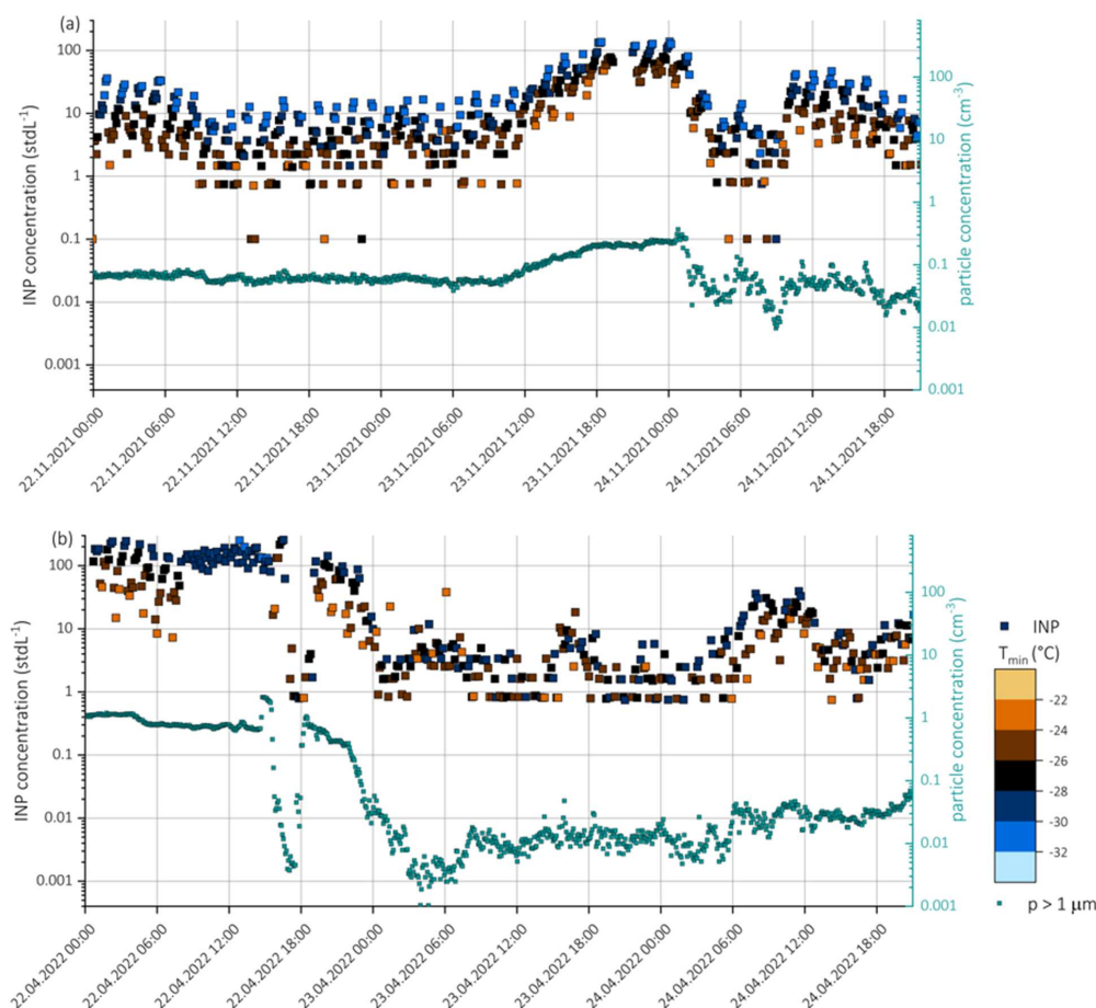
340 Figure 8: Timeseries of the INP concentration and aerosol particle concentration larger than 1 \mu\text{m} from November 22 nd to 24 th 2021 (panel a) and from April 22 nd to 24 th 2022 (panel b). Blue and brown colors present the nucleation temperature ( \pm 1 ^{\circ}\text{C} ), and green aerosol particle concentration larger than 1 \mu\text{m} . INP concentrations below the LOD are presented as values of 0.1 \text{stdL}^{-1} .
