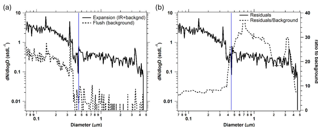
Figure 10: Average particle size distributions recorded downstream of the PCVI for 3784 PINE expansions and corresponding flush modes during nearly continuous operation from Feb 12 - 20. (Panel a) residuals plus background aerosol particles during expansion (solid line) and flush mode background particles (dashed line) at temperatures below -29 °C. (Panel b) residual size distribution after subtracting the background (solid, left axis) and the ratio of residuals to background particles (dashed, right axis). All concentrations are reduced by the PCVI concentrating factor of 27.5. Blue lines indicate the break between small and large particles (0.45 µm). Sizes are reported as PSL diameter.
