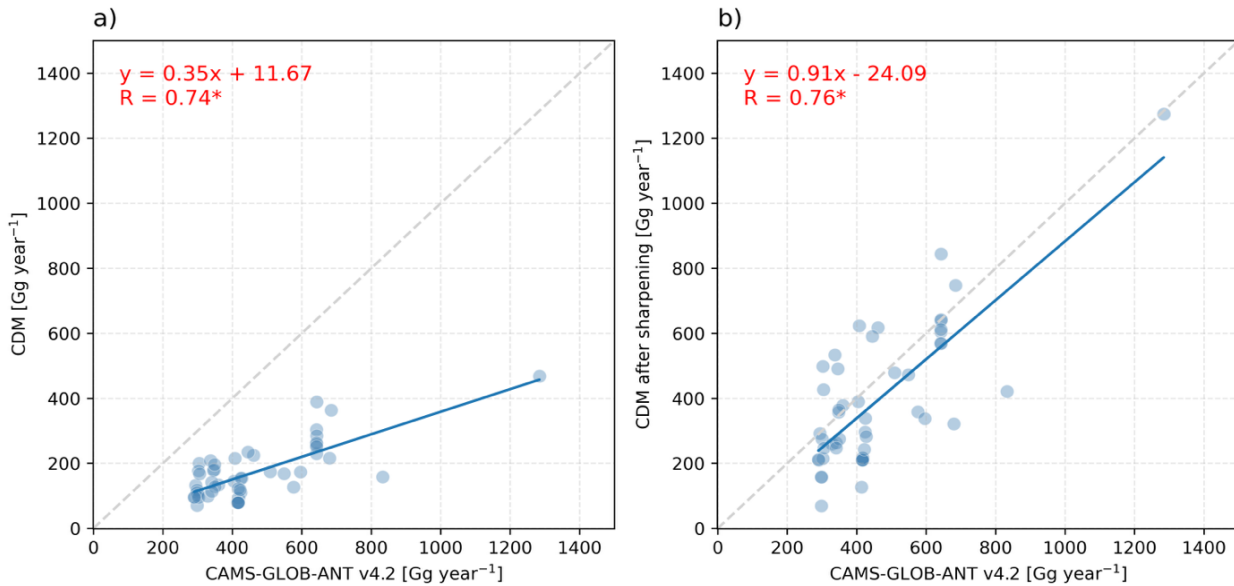
Figure 5. Comparison of SO 2 point source emissions between model input inventory (CAMS-GLOB-ANT v4.2, x axis) and model-based top-down estimate (y axis). The largest 50 point source emissions in CAMS-GLOB-ANT v4.2 are used in this comparison. a) y axis represents the top-down emissions derived from classic divergence method (CDM). b) y axis represents the top-down emissions from CDM sharpened by the 5 × 5 kernel. Since the top-down emission signal may be spatially shifted, the sum of emissions from two grid cells is used for comparison: one corresponding to the point source location and the other to the grid cell with the maximum emissions in the surrounding area.
