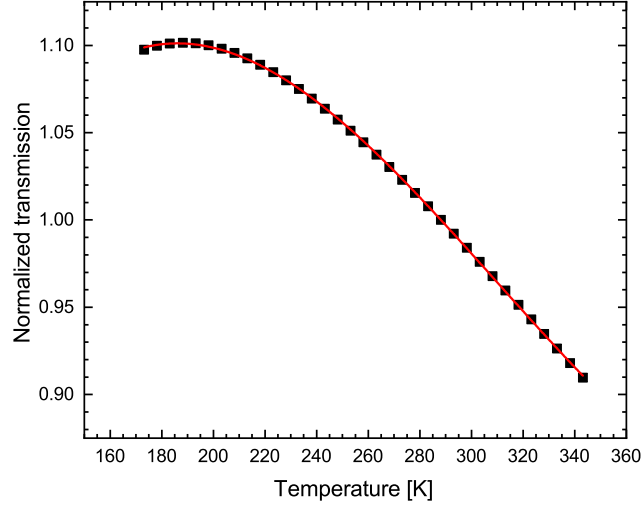
Figure A1. The temperature dependent transmission of the rotational Raman lines when applying both interference filters simultaneously. The transmission is normalized to a temperature of T_0 = 288.15 K. The polynomial fit curve to the data points is used to correct the rotational Raman signal for the temperature effect.
