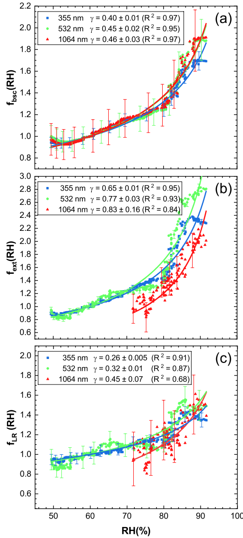
Figure 6. (a) Backscatter enhancement factor f_{\text{bsc}} , (b) extinction enhancement factor f_{\text{ext}} and (c) lidar ratio enhancement factor f_{\text{LR}} . A relative humidity (RH) of 60% is used to normalize the enhancement factors for all quantities except of the extinction coefficient and lidar ratio at 1064 nm, where 75% RH are used. The hygroscopic growth parameter \gamma at 355, 532 and 1064 nm is given for all quantities. Additionally, the R^2 value of the fit following equation 2 is listed. The uncertainty already includes the fit error and the uncertainty of the quantity itself (see last column of Table 2).
