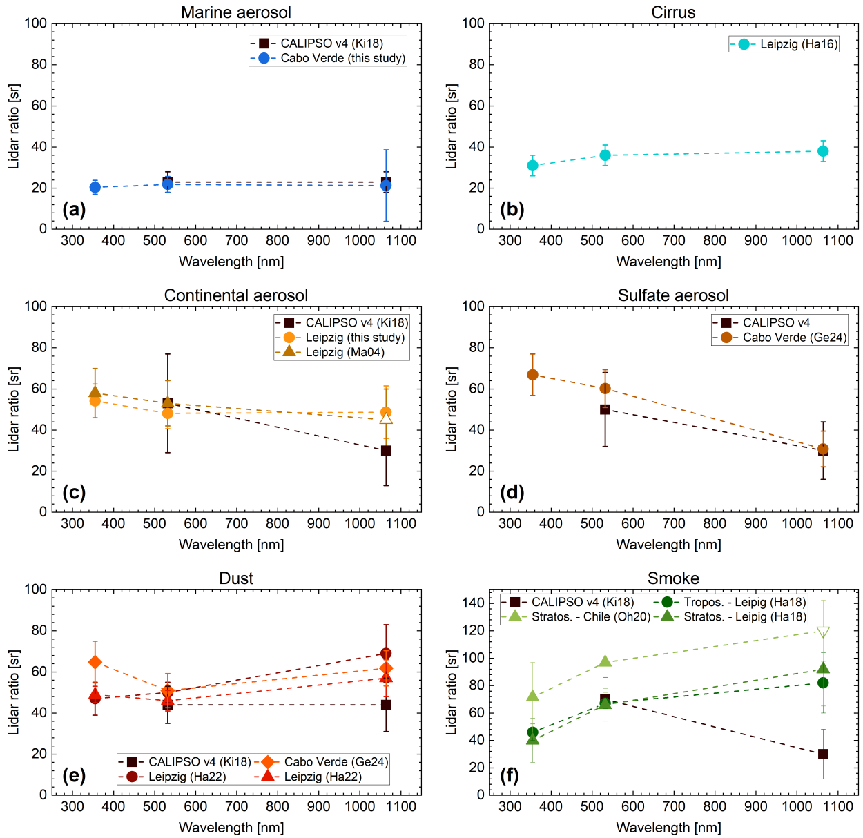
Figure 7. Spectral slope of the lidar ratio for (a) marine aerosol, (b) cirrus clouds, (c) continental aerosol, (d) sulfate aerosol, (e) mineral dust and (f) smoke (in the troposphere and stratosphere). The Raman lidar observations shown in filled colored symbols are compared to the assumptions made in the CALIPSO v4 aerosol typing and lidar ratio selection algorithm (black squares). Open symbols refer to a combination of lidar and photometer observations. The references are listed in Tab. 3 and the values are provided for convenience in Table 4 and separately for mineral dust in Table 5.
