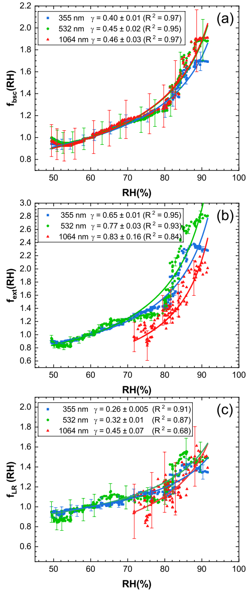
Figure 6. (a) Backscatter enhancement factor f_{\text{bsc}} , (b) extinction enhancement factor f_{\text{ext}} and (c) lidar ratio enhancement factor f_{\text{LR}} . A relative humidity (RH) of 60% is used to normalize the enhancement factors for all quantities except of the extinction coefficient and lidar ratio at 1064 nm, where 75% RH are used. The hygroscopic growth parameter \gamma at 355, 532 and 1064 nm is given for all quantities. Additionally, the R^2 value of the fit following equation 2 is listed. The uncertainty already includes the fit error and the uncertainty of the quantity itself (see last column of Table 2).
