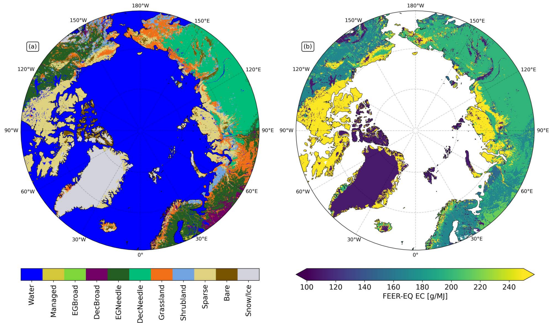
Supplementary Figure 1 for RC3: Comparison of Fire-biomes (a, shown in Figure 3b and Table A1 in the main manuscript), and associated FEER-Equivalent biome specific emission coefficients for CO ( EC_{CO}^b )
