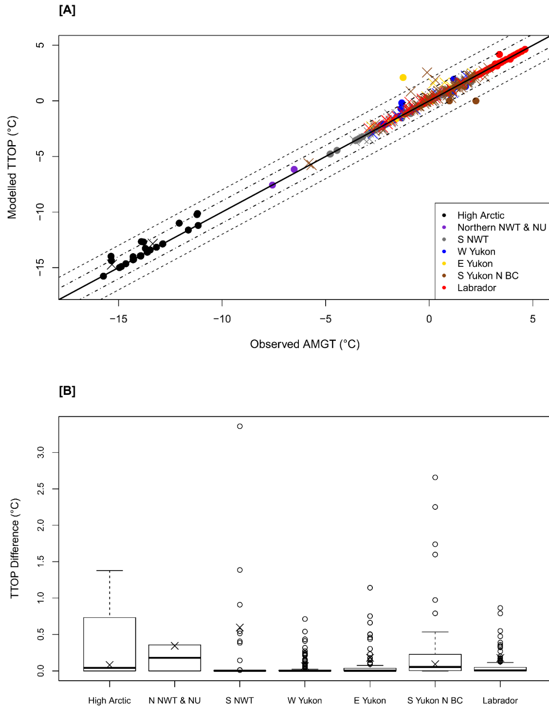
Figure S1. A) Comparison of TTOP model outputs to the measured annual mean ground temperature (AMGT) and B) boxplots for the absolute difference between the modelled TTOP and the measured AMGT close to the frost table across the entire study area and for individual regions. The solid line in panel A is the 1:1 relation between modelled and observed while the dashed lines indicate 1 and 2 °C differences.
