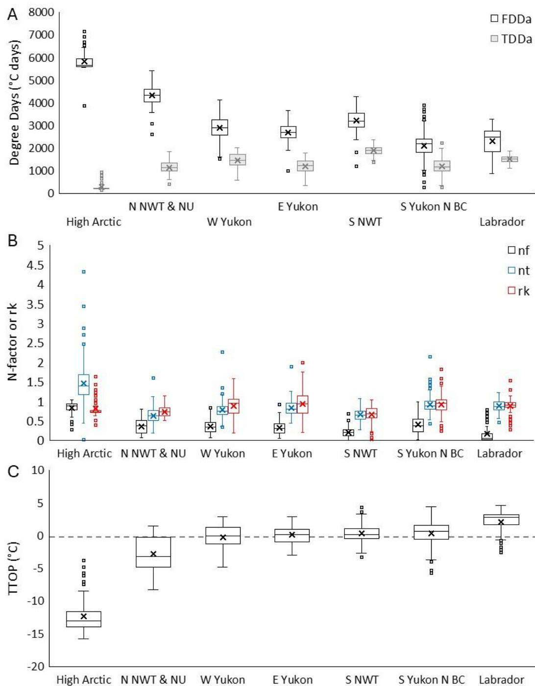
Figure S2. Boxplots for A) FDD a and TDD a , B) n f , n t , and r k and C) TTOP overall and for individual regions. Mean values are represented by an X. For some regions, maximum and minimum are shown by the ends of the whiskers. However, for some regions outliers are shown as circles after the whiskers and the ends of the whiskers instead show the value for one and a half times the interquartile range. The ends of the box show the first (25 percent) and third (75 percent) quartiles and the black line within the box shows the median.
