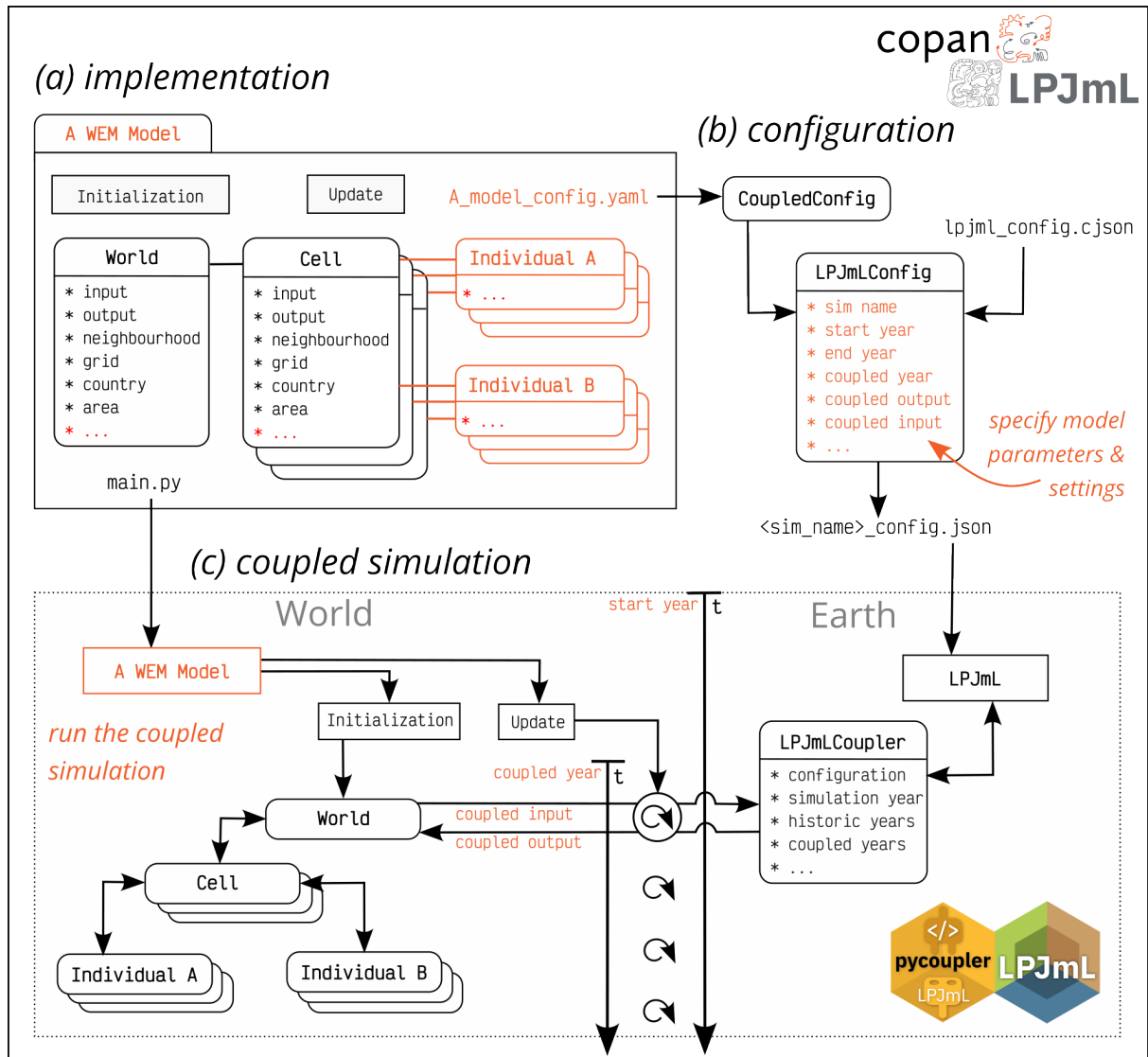
Figure 2. Stylised flow chart of the integrated copan:LPJmL WEM framework. The orange highlighting indicates the parts and attributes that can be modified, extended or added. This applies to each entity type represented within its structural hierarchy and modelling interfaces of the framework described in detail in Section 2.2. ‘A WEM model’ can be implemented by using and/or extending the World and corresponding Cell entities and by creating, for example, Individual A and B with distinct features and processes (a). The entities are hierarchically linked, while their interactions and processes are defined within the respective coupled model implementation. The three dots indicate that entities and attributes can be further extended. By creating A_WEM_model_config.yaml , those can be set up and added to the LPJmL configuration ( LPJmLConfig ) in which further simulation parameters and settings are specified (b). The coupled simulation is started based on the generated <sim_name>_config.json file (c). The LPJmLCoupler handles the coupling between LPJmL (Earth) and ‘A WEM model’ by receiving and sending coupled data on an annual basis. The circular arrows represent the annual exchange of coupled LPJmL input and output data. ‘A WEM model’ can compute intra-annual processes based on coupled LPJmL output to generate new coupled LPJmL input for closed feedback loops throughout the simulation period.
