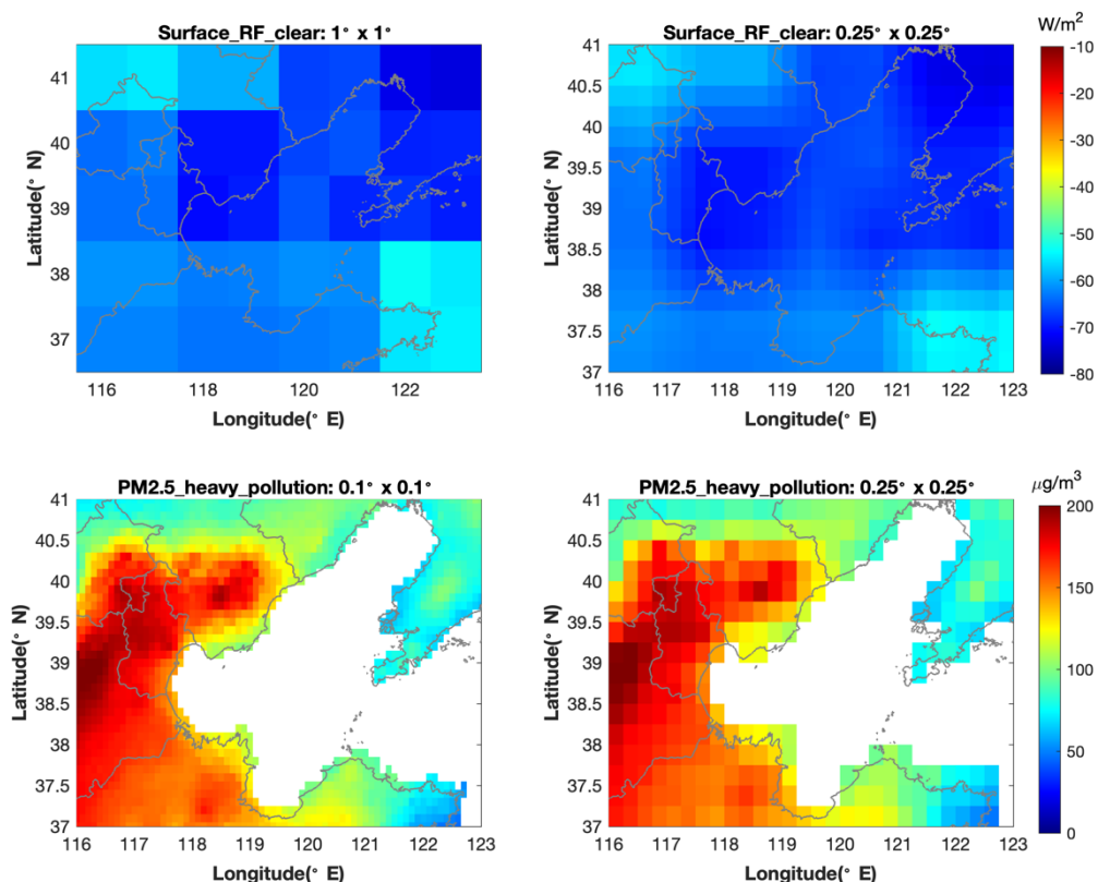
Figure S1. The comparison between the original data (first column) and the interpolated data (second column) in the study area. The first row is the radiative forcing (RF) from CERES at the surface in clear sky, and the second row is the interpolation for the PM 2.5 from TAP.
