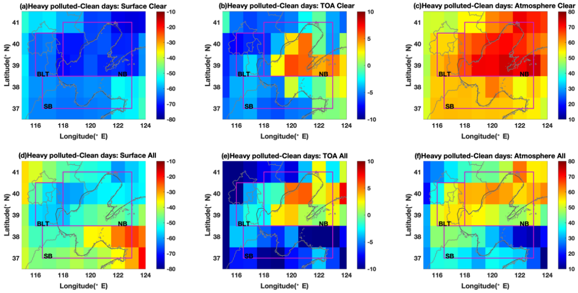
Figure 4. The short-wave radiative forcing ( \text{Wm}^{-2} ) on regional \text{PM}_{2.5} heavy pollution days calculated from the difference between CERES net radiative fluxes on regional heavy pollution days and the mean of clean days for all stations: (a and d) at the surface; (b and e) at the top of atmosphere (TOA); (c and f) in the atmosphere, in clear sky (a-c) and all sky (d-f).
