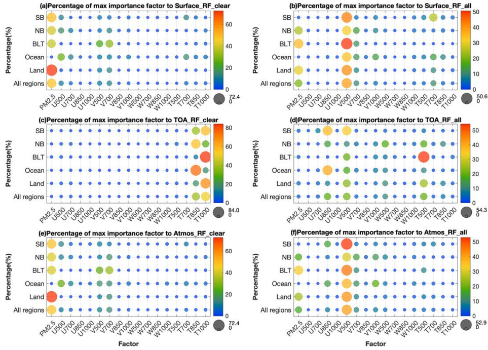
Figure 9. The percentage of regional grids with maximum importance factor (including PM_{2.5} , winds, and temperature at four levels) to the radiative forcing on regional heavy pollution days for surface (first row: a and b), TOA (second row: c and d), and atmosphere-Atmos (third row: e and f) in clear sky (first column: a, c, and e) and all sky (second column: b, d, and f) in different regions. The x-axis indicates different impact factors, while the y-axis denotes different regions. The larger the circle and the redder the color, the higher the percentage. Conversely, the smaller the circle and the bluer its color, the closer the percentage is to 0.
