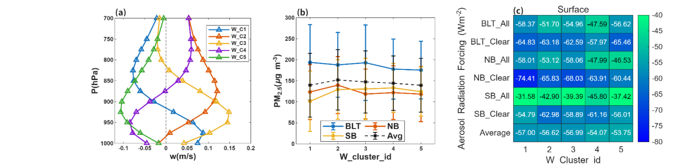
Figure 7. The five vertical wind profiles under 850 hPa by k-means clustering on the regional heavy pollution days: (a) the w wind, (b) the PM 2.5 concentrations, and (c) the radiative forcing in the three regions in clear- and all-sky at the surface.
