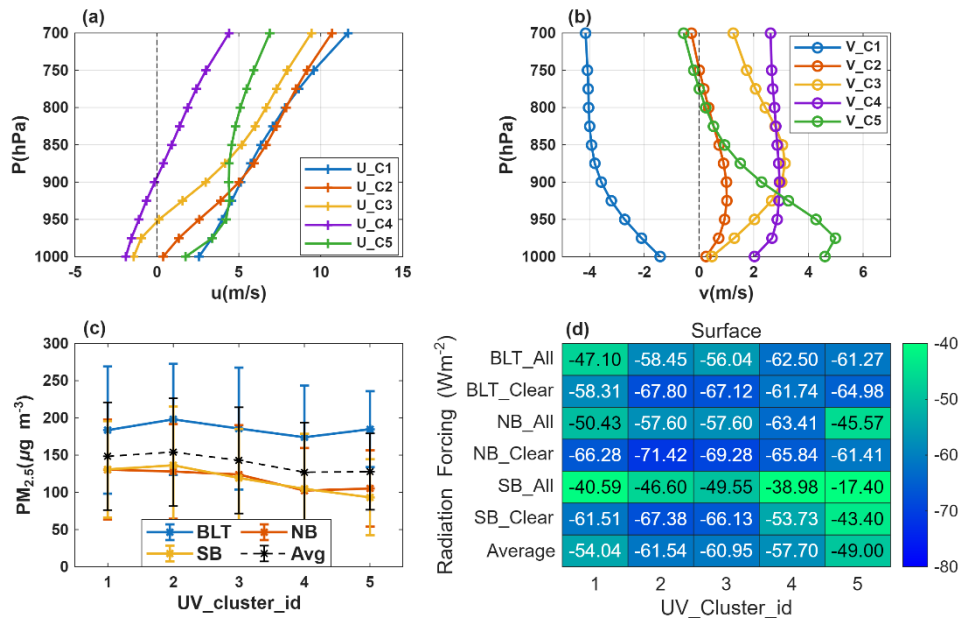
Figure 6. The five horizontal wind profiles under 850 hPa by k-means clustering on the regional heavy pollution days: (a) u wind, (b) v wind, (c) the PM 2.5 concentrations, and (d) the radiative forcing in the three regions in clear- and all-sky at the surface at the five clusters.
