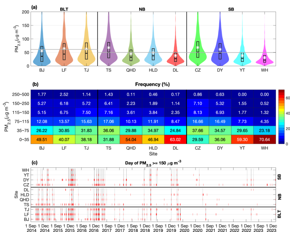
Figure 3. The statistics of PM 2.5 concentration at the stations in the Bohai Rim in autumn and winter during 2014-2023: (a) Violin plot of daily PM 2.5 , the mean PM 2.5 (white asterisk) at sites and subregions (gray line); (b) Frequency distribution of PM 2.5 at stations; (c) The heavy pollution day at each station (red) and for each region (gray).
