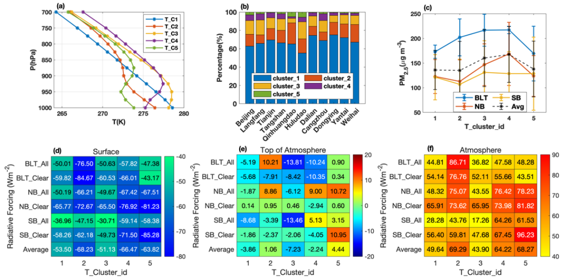
Figure 5. The five temperature (T) profiles under 850 hPa by k-means clustering on the regional heavy pollution days (a); their statistics at the 11 stations (b); the PM 2.5 concentration (c) and the radiative forcing in the three regions in clear- and all-sky at the surface (d), top of atmosphere (e), and in the atmosphere (f) at the five T clusters.
