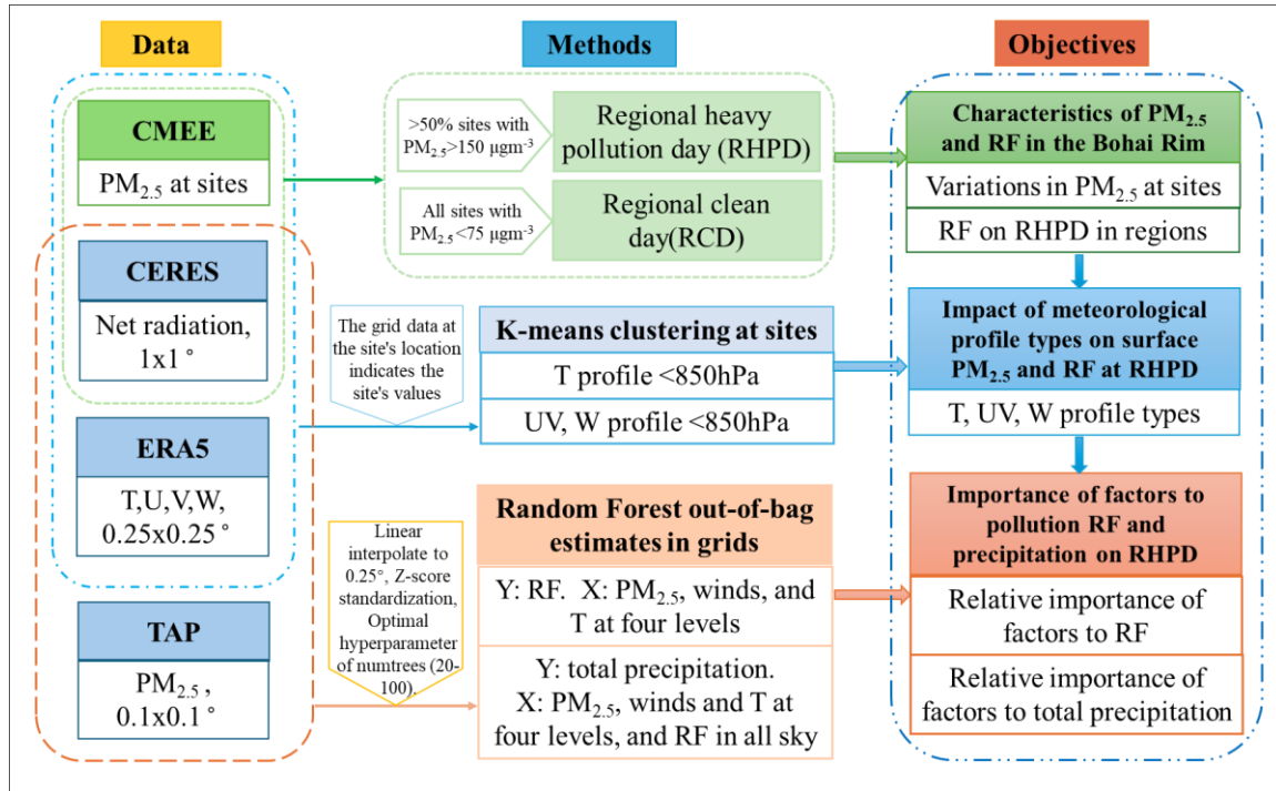
Figure 2. The data usage workflow and framework in this work.
