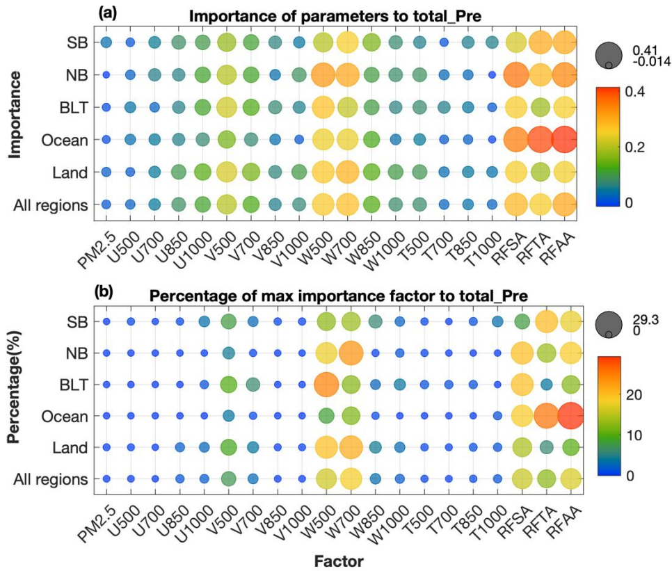
490 Figure 10. (a) The Random Forest’s importance of PM 2.5 , winds, and temperature at four levels, and RF in all-sky to total precipitation; and (b) the percentage of regional grids with maximum importance factor to total precipitation on regional heavy pollution days in different regions.
