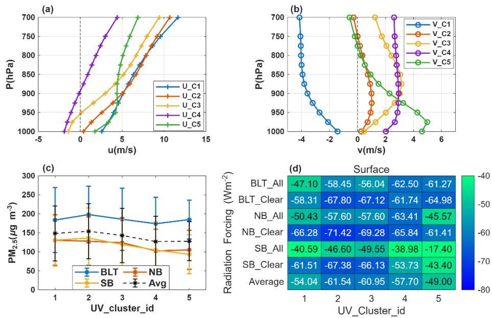
Figure 6. The five horizontal wind profiles under 850 hPa by k-means clustering on the regional heavy pollution days: (a) u wind, (b) v wind, (c) the PM_{2.5} concentrations, and (d) the radiative forcing in the three regions in clear- and all-sky at the surface at the five clusters.
