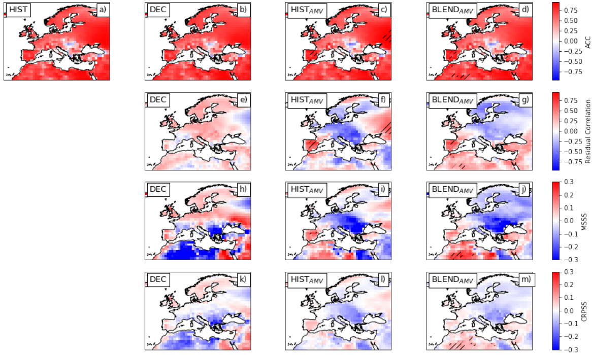
430 Figure 6: ACC (a–d), Residual correlation(e–g), MSSS (h–j), and CRPSS (k–m) calculated from 10-year forecasts of winter surface temperature over the evaluation period 1966–2000 for HIST (a), DEC (b, e, h, k), \text{HIST}_{\text{AMV}} (c, f, i, l), and \text{BLEND}_{\text{AMV}} (d, g, j, m). For \text{BLEND}_{\text{AMV}} , the summer surface temperature averaged over MED is used for the second-step selection. Hatched regions indicate significant improvement in comparison to randomly drawn subsets of 435 HIST (see Section 2.4).
