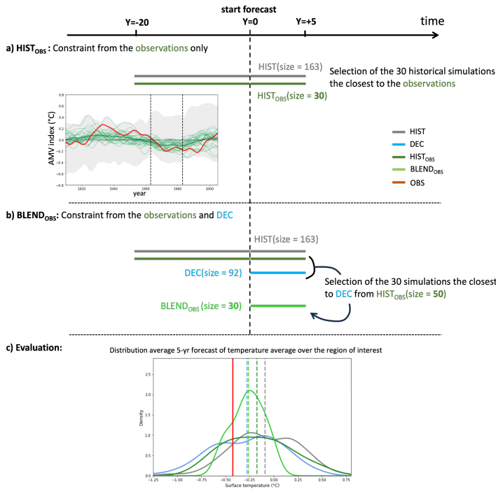
Figure 1. Diagram illustrating the concept and two types of dataset derived from the blending method. For both the historical (HIST) (Table 1) and hindcast (DEC) (Table 2) simulations, the datasets combine all the models (see Section 2.1). In the development of HIST_OBS (a) the AMV index (see section 2.2) from the historical simulations (minimum and maximum in gray) is compared to the ERSSTv5 observational dataset (green line), with the selection of the best 20 members in green. In the development of BLEND_OBS (b), a first selection of 50 members is then refined to 30 members. The histogram and the ensemble mean (vertical dashed line) of average 5-yr forecast surface temperature from the different datasets are evaluated against the ERA5 reanalysis (red line) (c).
