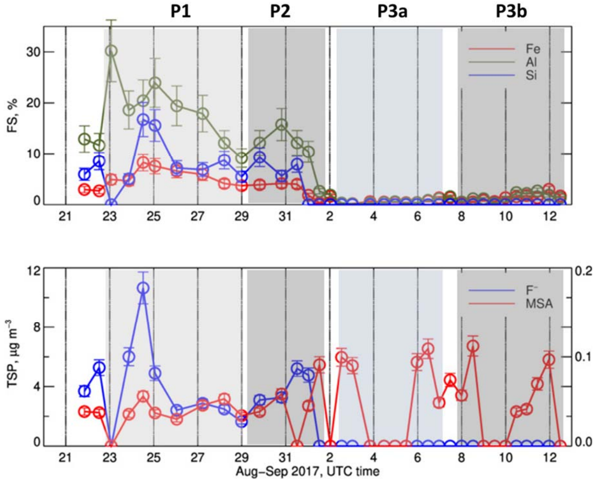
Figure 7. Top panel: Time series of the fractional solubility Al, Si and Fe in the TSP fraction. Bottom panel: Time series of concentrations of \text{F}^- (blue) and MSA (red) in the TSP fraction. The MSA concentrations are reported on the right axis of lower panel. Missing data correspond to periods when the measured concentrations were below the detection limit.
