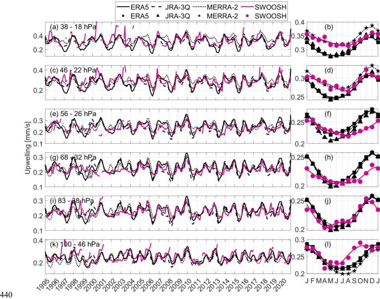
440 Figure 9: The same as Fig. 8, but for SWOOSH upwelling.
