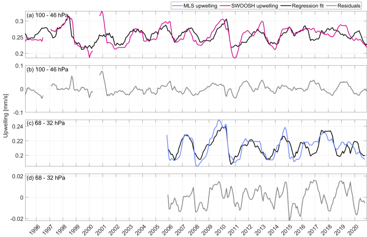
Figure 3: Time series of regression fits and residuals for (a)-(b) regression of 100-46 hPa SWOOSH upwelling, and (c)-(d) regression of 68-32 hPa MLS upwelling. Note the different vertical scaling for each panel. Uncertainty shading is omitted here to simplify the figure.
