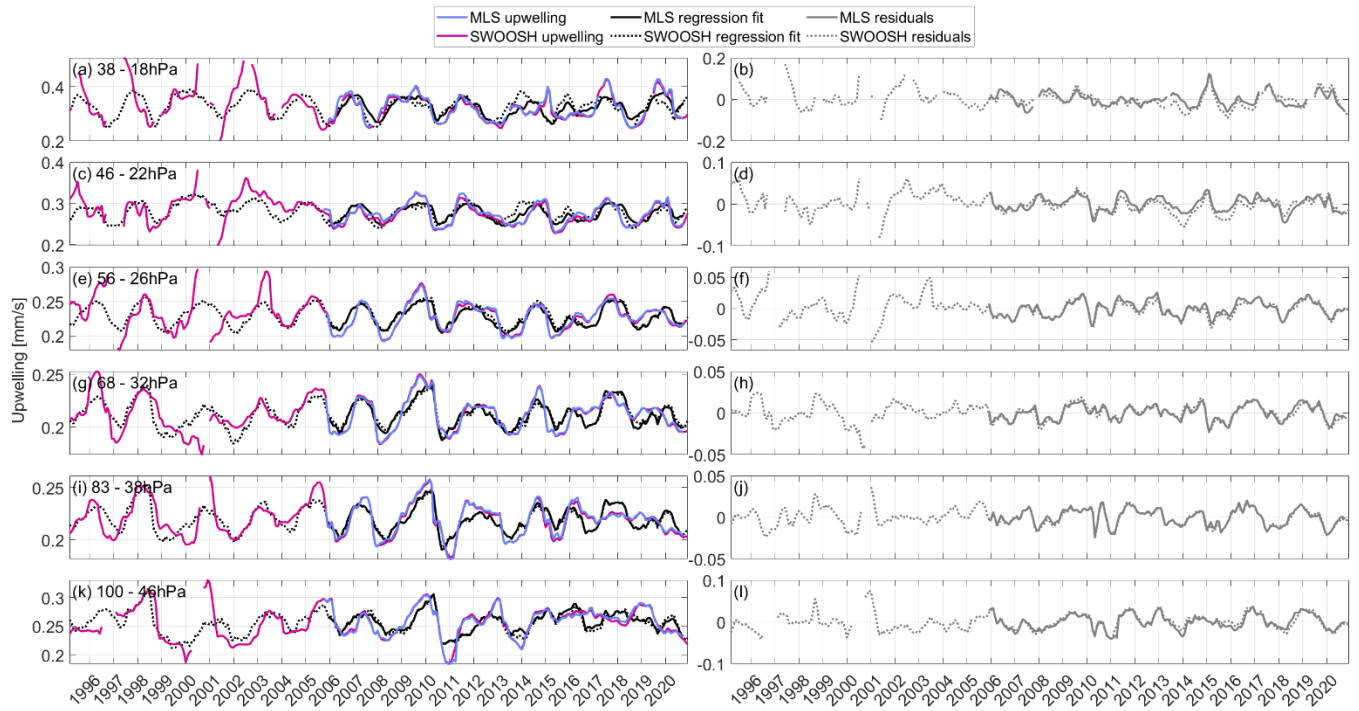
Figure A1: Time series of regression fits and residuals for MLS and SWOOSH at (a)-(b) 38-18hPa, (c)-(d) 46-22 hPa, (e)-(f) 56-26 hPa, (g)-(h) 68-32 hPa, (i)-(j) 83-38 hPa, and (k)-(l) 100-46 hPa.
