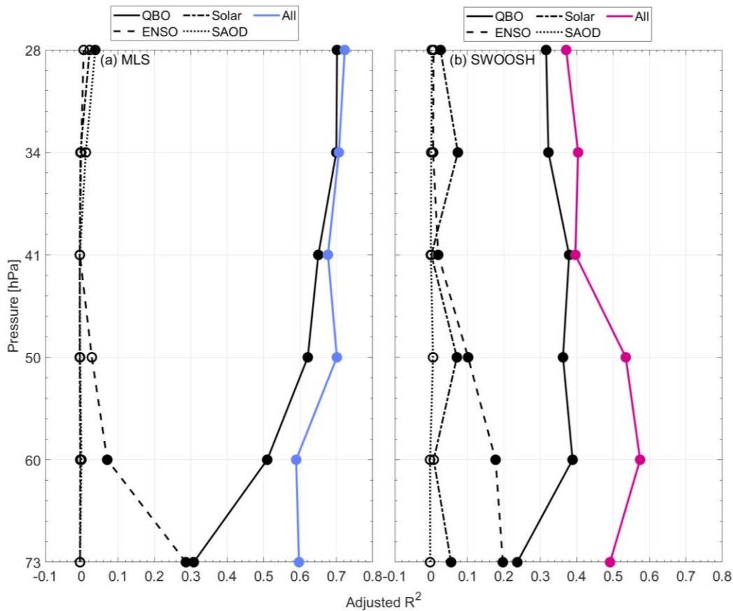
Figure 4: Profile of regression model adjusted R^2 for (a) MLS method upwelling and (b) SWOOSH method upwelling. Filled and unfilled circles represent significance and insignificance at the 95% level, respectively.
