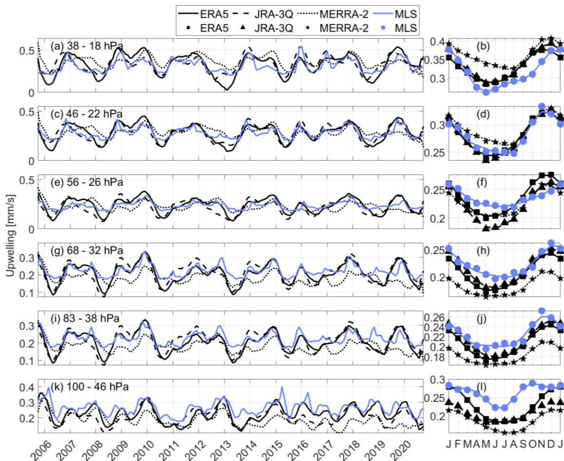
Figure 8: Tropical upwelling time series and corresponding seasonal cycle for upwelling calculated from MLS and the vertical component of the residual circulation from ERA5, JRA-3Q, and MERRA-2, for (a)-(b) 38-18 hPa, (c)-(d) 46-22 hPa, (e)-(f) 56-26 hPa, (g)-(h) 68-32 hPa, (i)-(j) 83-38 hPa, and (k)-(l) 100-46 hPa. Uncertainty shading is omitted here to simplify the figure.
