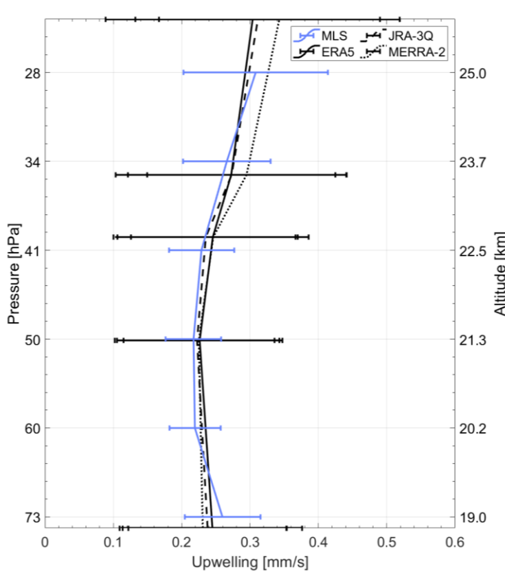
Figure 7: Climatological mean profile of upwelling from the MLS 12-month lagged correlation method and reanalysis vertical residual velocities. Horizontal bars give the uncertainty range derived as the 2\sigma standard deviation of the monthly time series.
