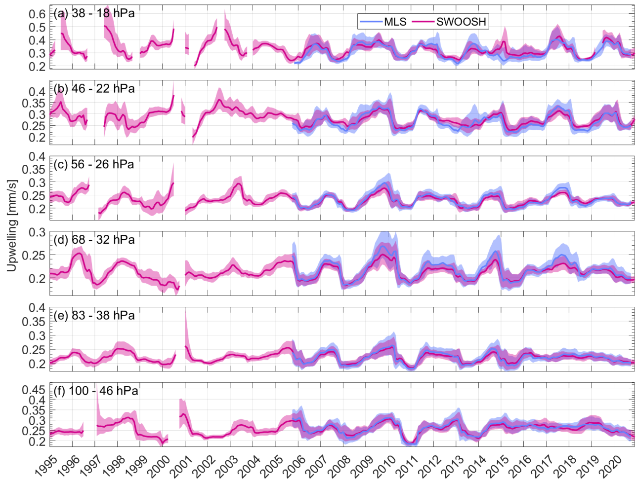
Figure 2: Time series of upwelling calculated from 12-month correlations of MLS and SWOOSH water vapour for (a) 38-18 hPa, (b) 46-22 hPa, (c) 56-26 hPa, (d) 68-32 hPa, (e) 83-38 hPa, and (f) 100-46 hPa. Shading indicates time-dependent error bars of the upwelling estimates calculated from the 95% confidence interval of the correlation coefficients.
