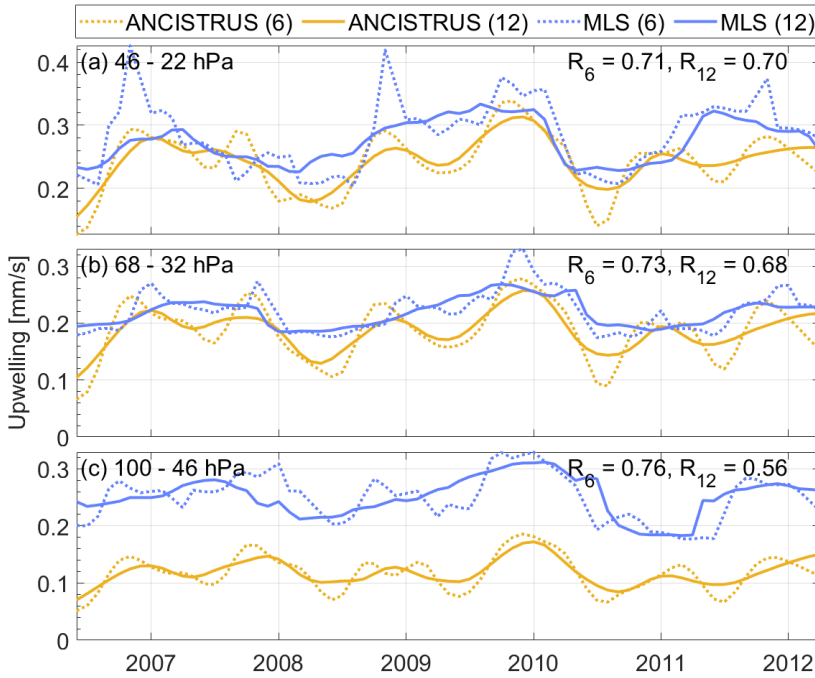
Figure 11: Time series of upwelling from ANCISTRUS and the MLS method for (a) ANCISTRUS at 24 km and MLS over 46-22 hPa (midpoint of about 24 km), (b) ANCISTRUS at 21 km and MLS over 68-32 hPa (midpoint of about 21 km), and (c) ANCISTRUS at 18 km and MLS over 100-46 hPa (midpoint of about 19 km). Uncertainty shading is omitted here to simplify the figure. The labels (6) and (12) in the legend denote the 6-month and 12-month methods for the MLS data, and corresponding smoothing in the ANCISTRUS data.
