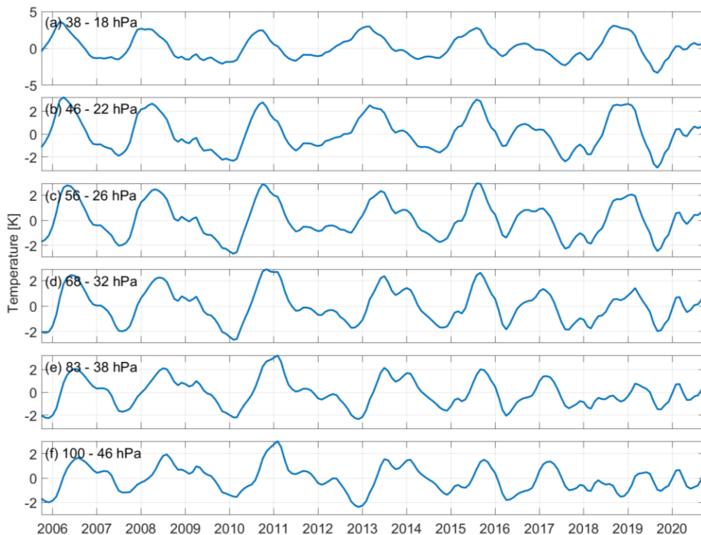
Figure 6: Detrended MLS temperature anomaly time series for the averaged levels (a) 38-18 hPa, (b) 46-22 hPa, (c) 56-26 hPa, (d) 68-32 hPa, (e) 83-38 hPa, and (f) 100-46 hPa.
