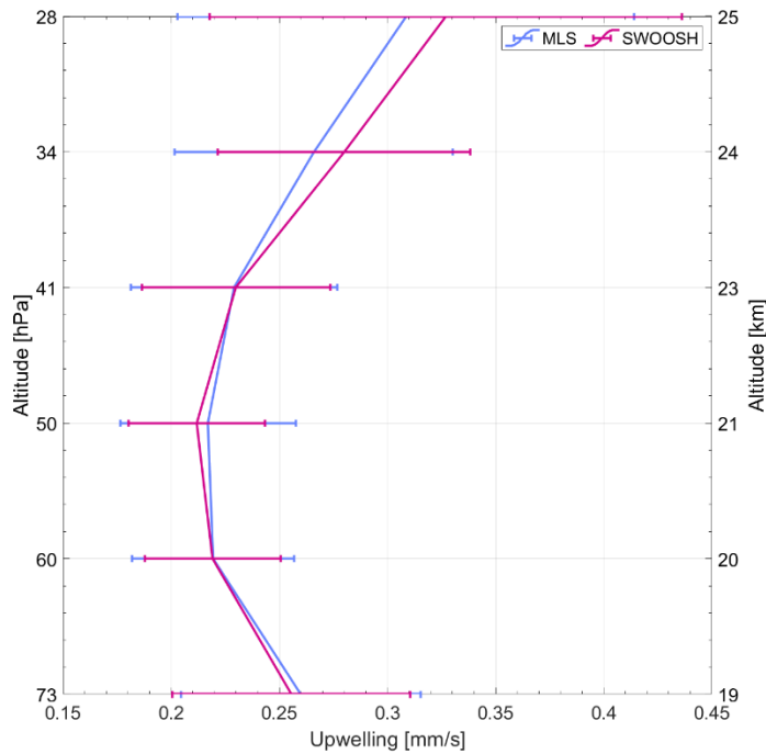
Figure 1: Profile of climatological mean tropical upwelling calculated from MLS and SWOOSH water vapour in the lower stratosphere. Horizontal bars give the uncertainty range derived as the 2\sigma standard deviation of the monthly time series.
