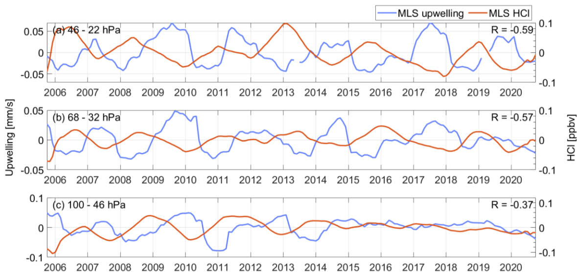
Figure B2: Time series of upwelling anomalies from MLS plotted along with HCl anomalies from MLS for (a) upwelling between 46-22 hPa and HCl at 22 hPa; (b) upwelling between 68-32 hPa and HCl at 32 hPa; and (c) upwelling between 100-46 hPa and HCl at 46 hPa.
