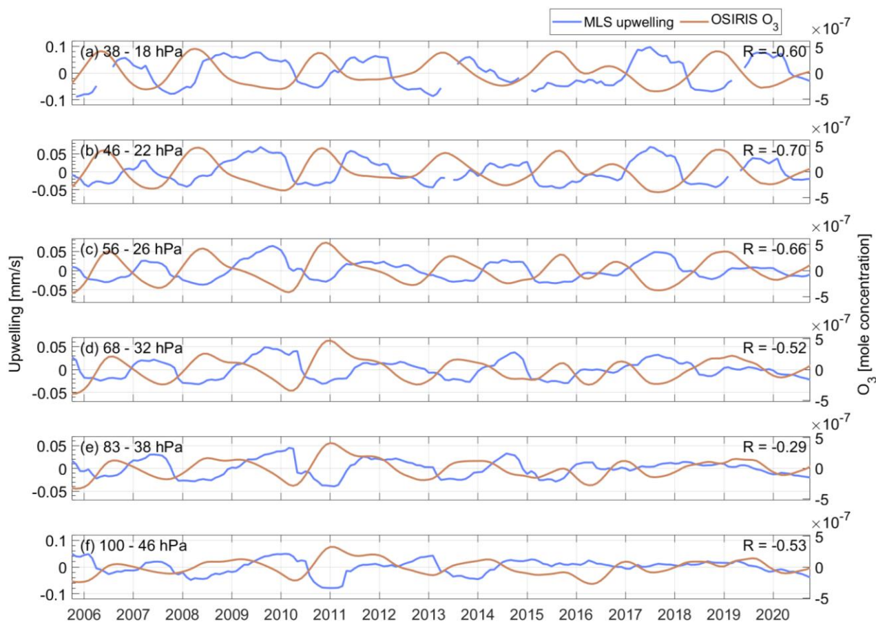
Figure B1: Time series of upwelling anomalies from MLS plotted along with O 3 anomalies from OSIRIS for (a) MLS between 38-18 hPa and OSIRIS O 3 between 22.5-27.5 km (about 38-18 hPa); (b) MLS between 46-22 hPa and OSIRIS O 3 between 21.5-26.5 km (about 44-20 hPa); (c) MLS between 56-26 hPa and OSIRIS O 3 between 20.5-24.5 km (about 52-27 hPa); (d) MLS between 68-32 hPa and OSIRIS O 3 between 18.5-23.5 km (about 73-33 hPa); (e) MLS between 83-38 hPa and OSIRIS O 3 between 17.5-22.5 km (about 87-37 hPa); and (f) MLS between 100-46 hPa and OSIRIS O 3 between 16.5-21.5 km (about 103-45 hPa).
