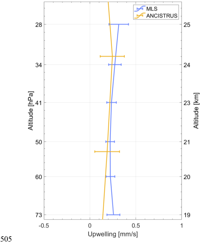
505 Figure 10: Profile of upwelling for ANCISTRUS and the MLS method. Horizontal bars give the uncertainty range derived as the 2\sigma standard deviation of the monthly time series.
